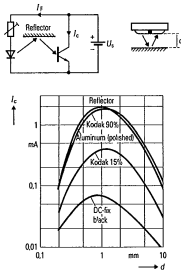
Fig. 5 SFH 900 collector current I_C as a function of reflector distance d with different reflector materials
