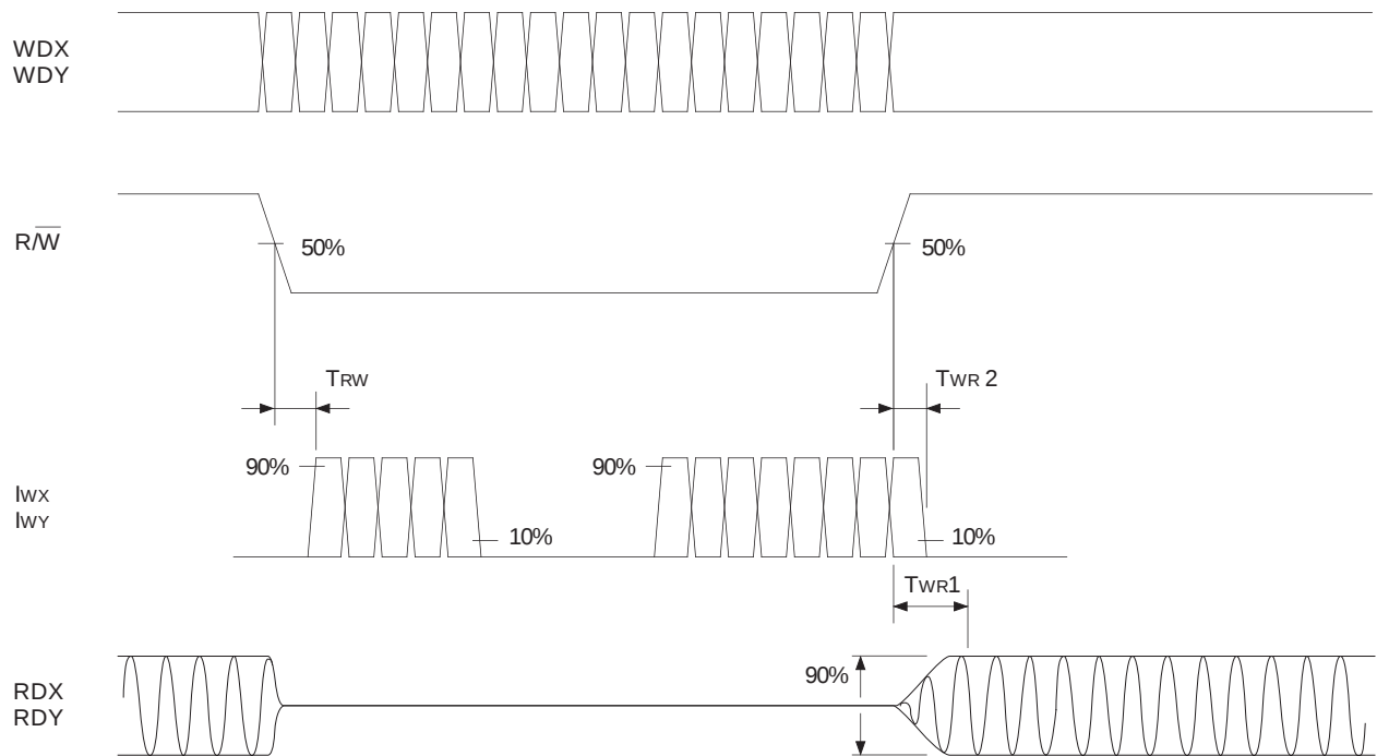
Timing Chart 1
