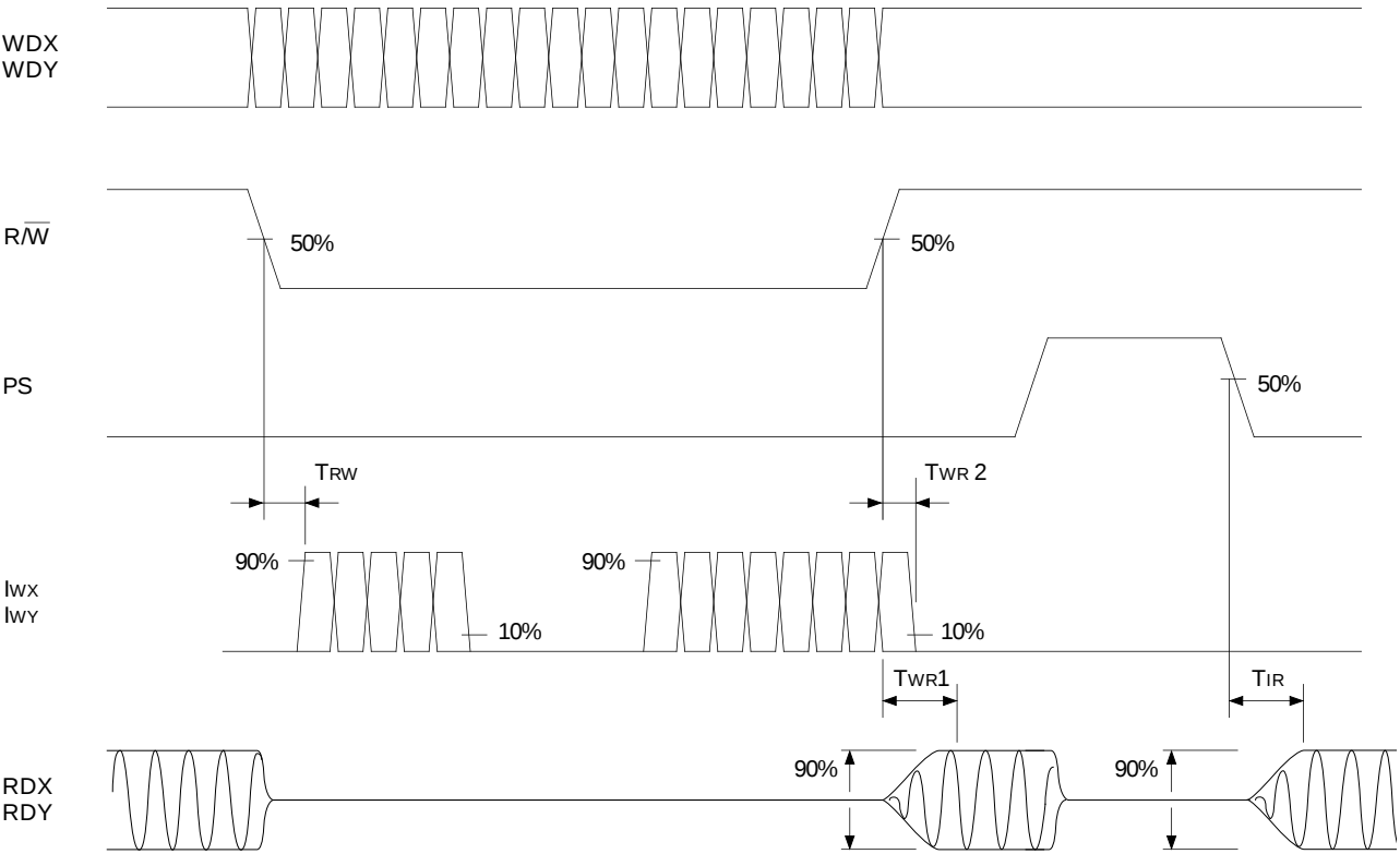
Timing Chart 1
