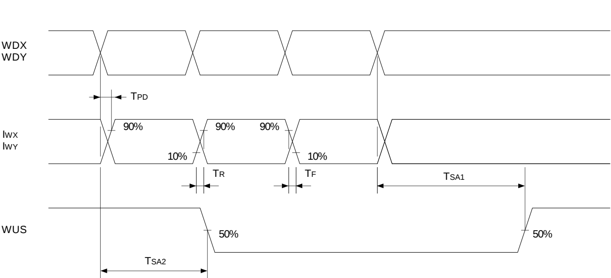
Timing Chart 2
