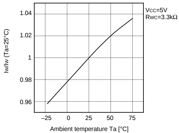
Normalized write current vs. Ambient temperature
