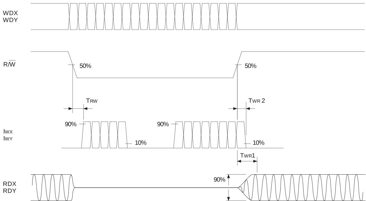
Timing Chart 1
