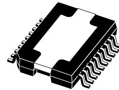
PowerSO-20 slug-up
