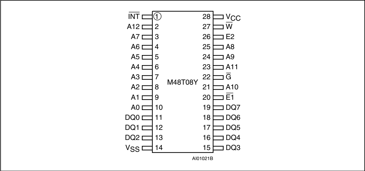
Figure 3. SOIC connections
