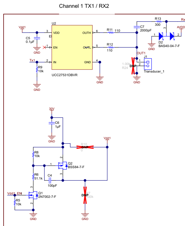
Figure 27. TDC1000-BSTEVM
