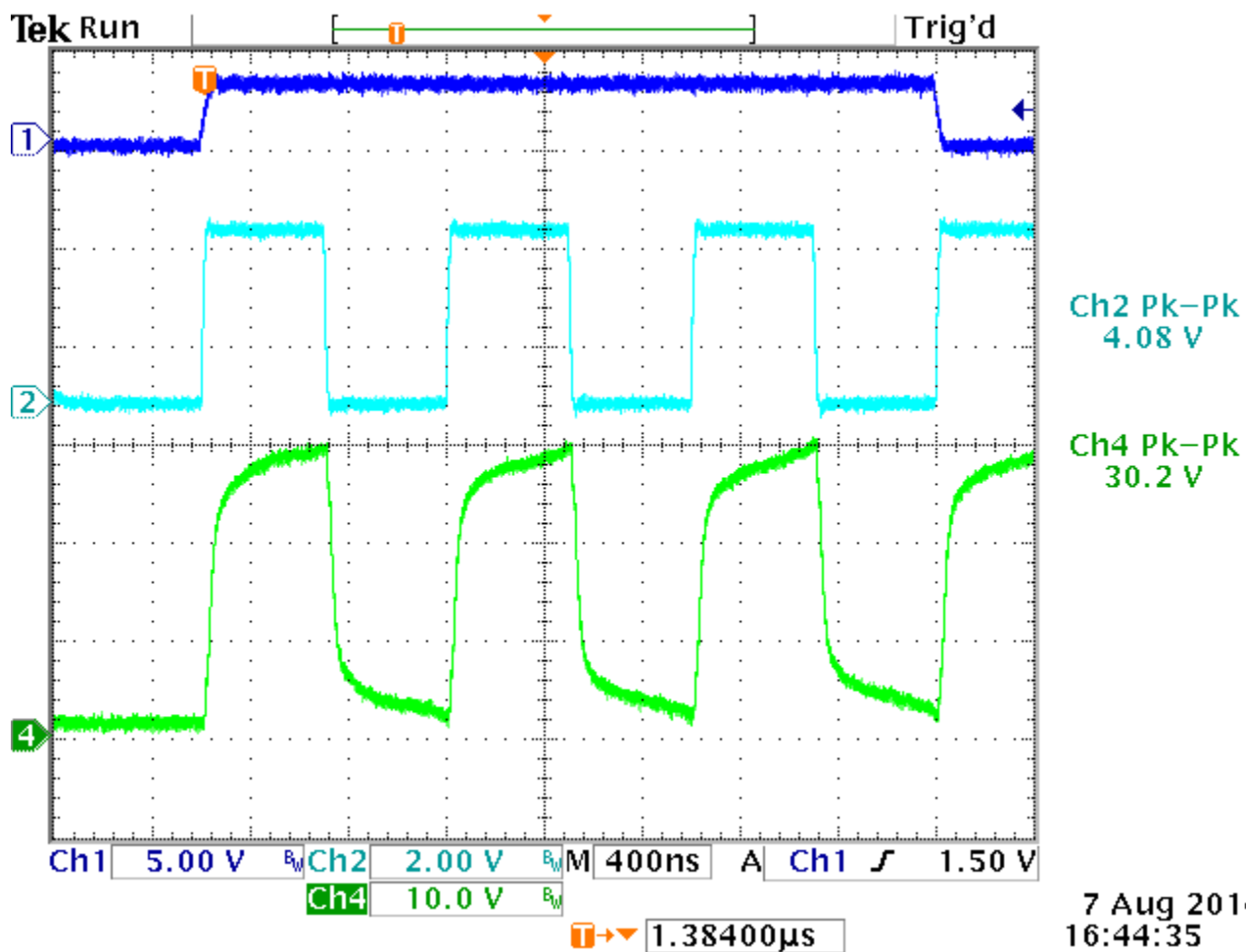
Figure 7. Top to Bottom: TDC1000's START Pulse (Dark Blue), TDC1000's Tx Signal (Light Blue), and the Boosted 30 V of TD1000's Tx Signal (Green)
