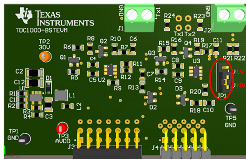
Figure 12. Jumper
