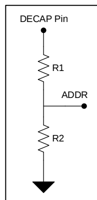
Figure 4. External Resistor Connection Diagram for the ADDR Pin
