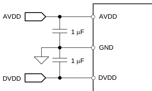
Figure 140. Power-Supply Decoupling
