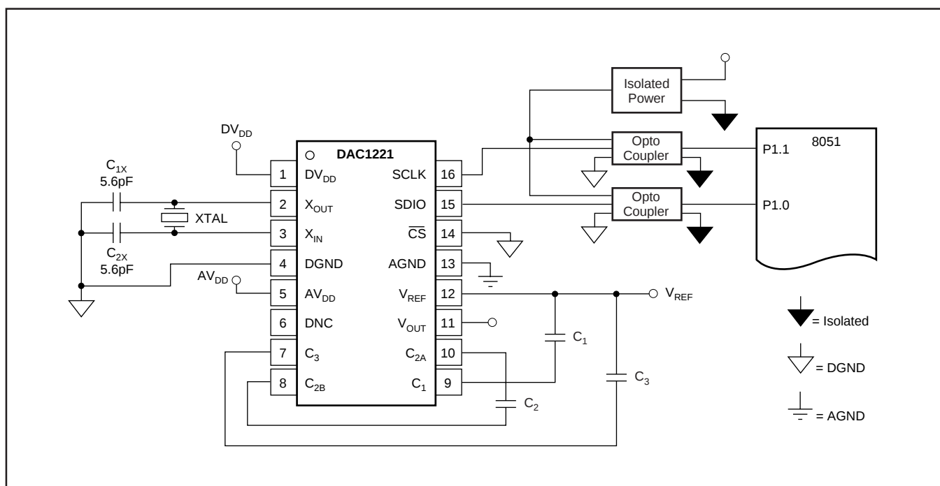
FIGURE 4. Isolation for Two-Wire Interface.
