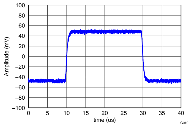
Figure 51. Small-Signal Response Over Capacitive Loads ( G = 1 )
