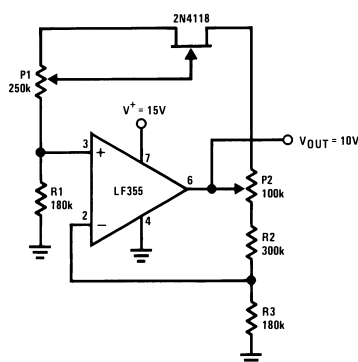
Figure 43. Low Drift Adjustable Voltage Reference
