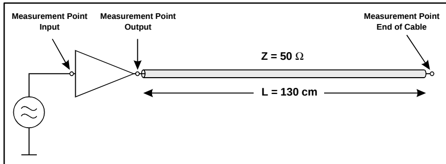
Figure 59. Setup for Obtaining Output Waveforms
