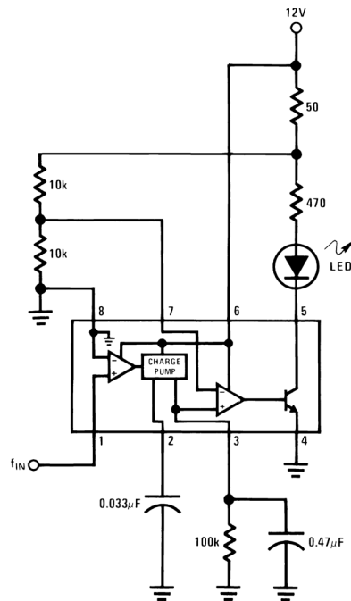
Figure 34. Frequency Switch With Resistor Divider Threshold
