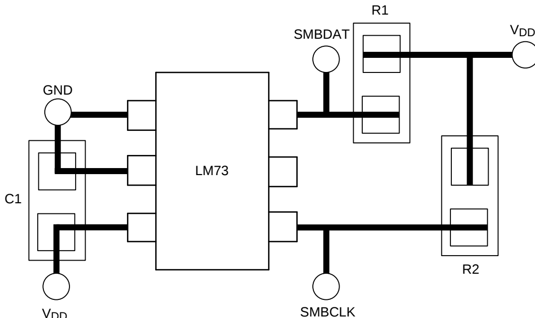
Figure 16. PBC Layout
