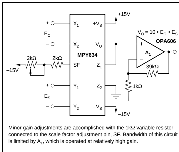
FIGURE 7. Voltage-Controlled Amplifier.
