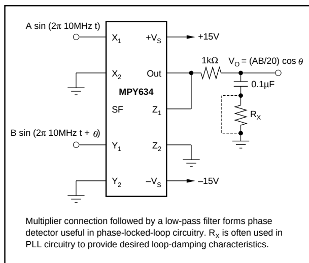
FIGURE 6. Phase Detector.
