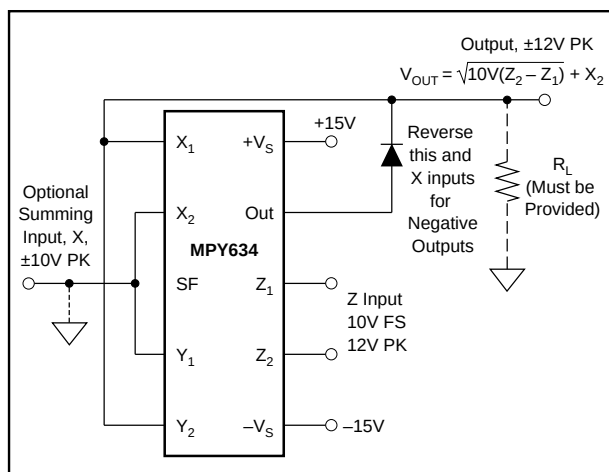
FIGURE 5. Square-Rooter Connection.
