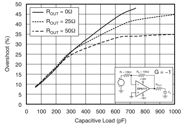
Figure 39. Small-Signal Overshoot vs Capacitive Load (100-mV Output Step)
