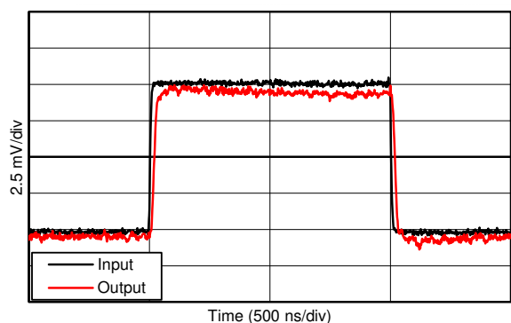
Figure 7-28. Positive Overload Recovery
