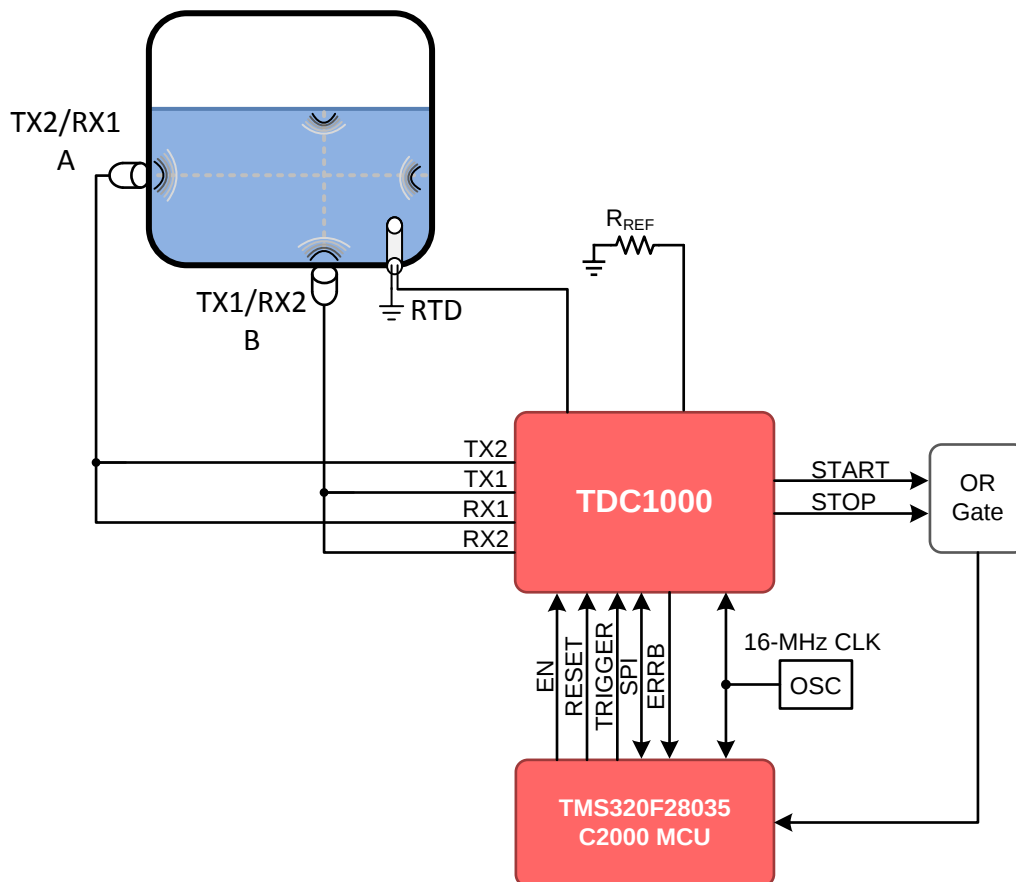
Figure 51. Level and Concentration Measurement Application Diagram
