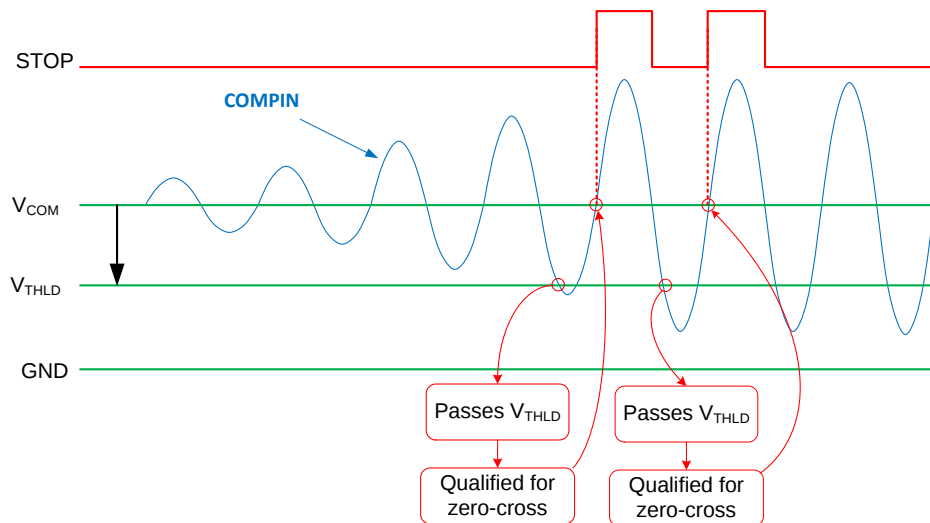
Figure 22. Signal Qualification, Zero-cross Detection and STOP Pulse Generation
