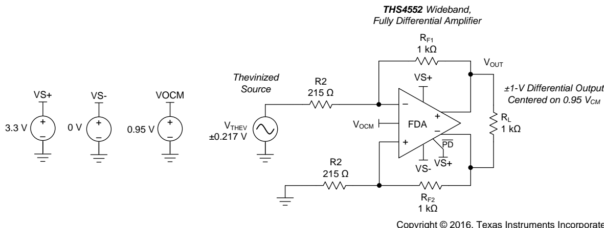
Figure 72. Input V_{ICM} Analysis Circuit From the Design of Figure 96
