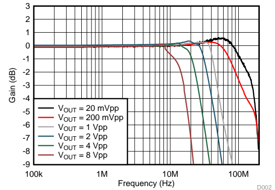
Figure 2. Frequency Response vs V_{\text{OUT}}
