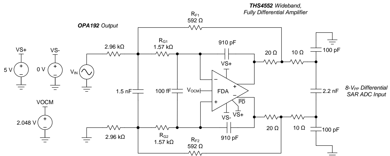
Figure 90. Example 100-kHz Butterworth Filter
