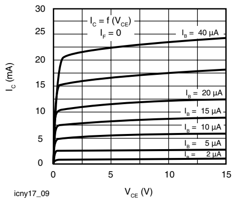
Fig. 9 - Transistor Characteristics
