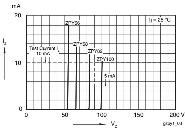
Figure 9. Breakdown Characteristics
