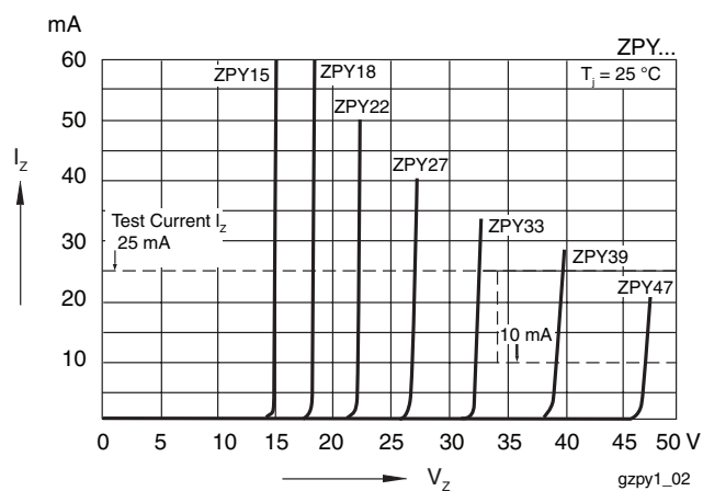
Figure 8. Breakdown Characteristics
