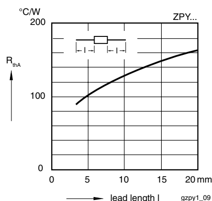
Figure 6. Thermal Resistance vs. Lead Length
