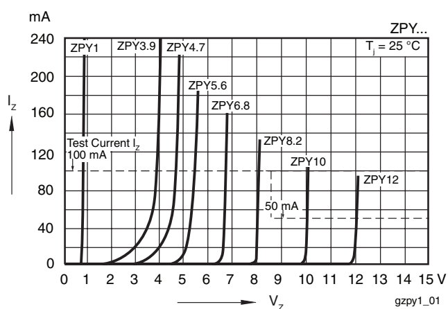
Figure 7. Breakdown Characteristics
