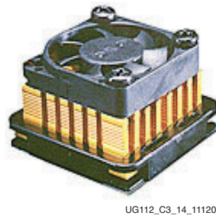
Figure 3-14: Example of Active Heatsink for BGA (Malico)
