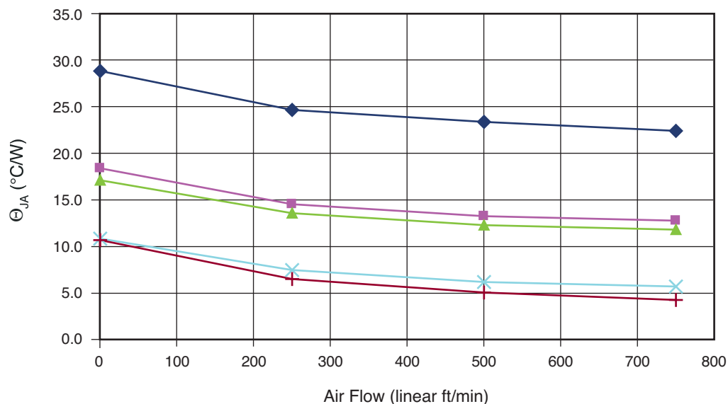
Figure 3-9: Effect of Active and Passive Heat Sinks on the Thermal Resistance ( \theta_{JA} ) of PG299 Packages
