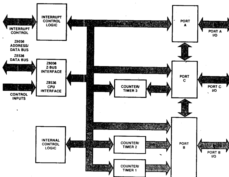
Figure 1-1. Z8036/Z8536 Z-CIO/CIO Block Diagram
