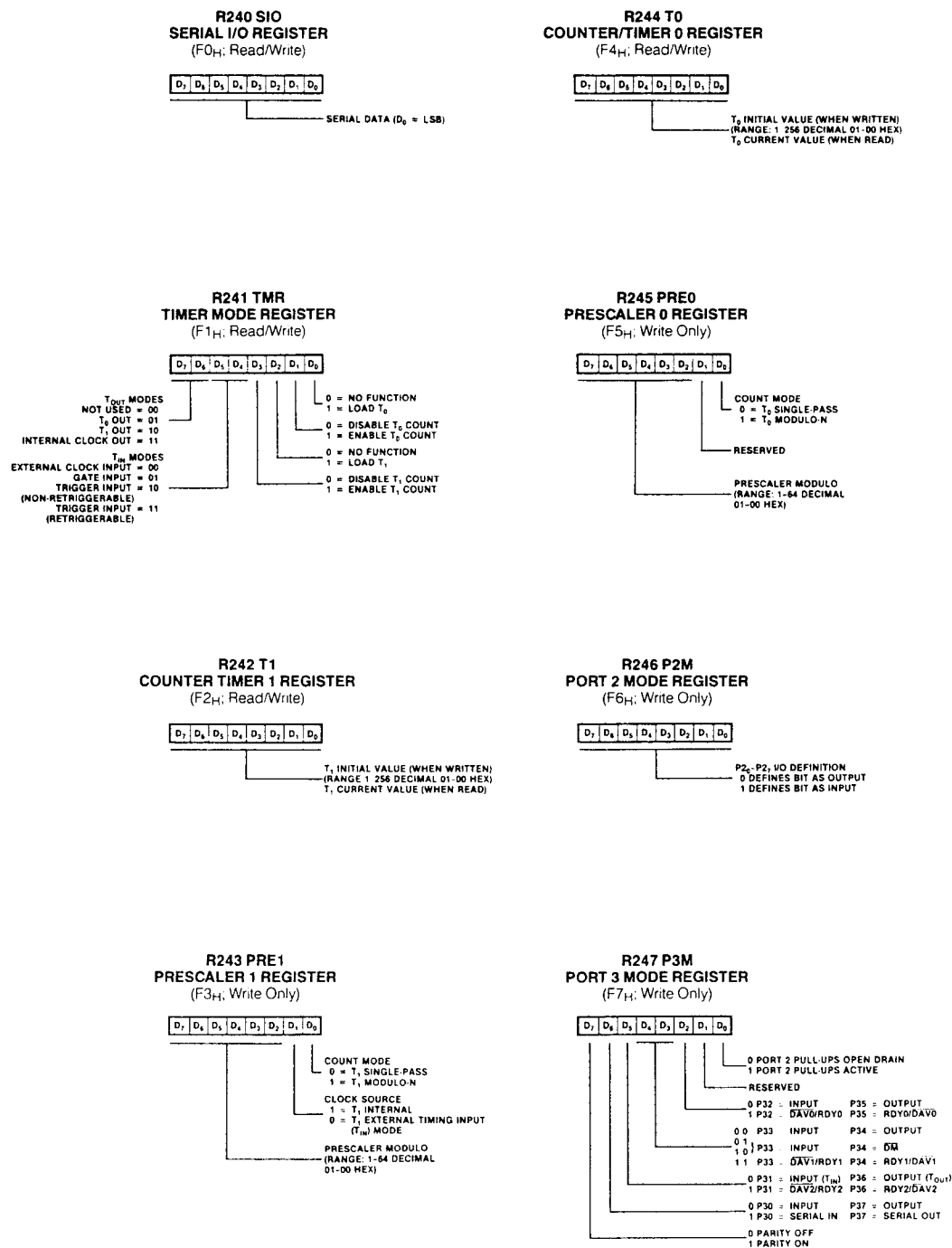
Figure 11. Control Registers
