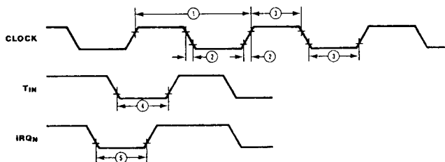
Figure 14. Additional Timing
