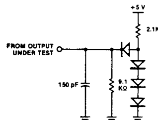
Figure 12. Test Load 1
