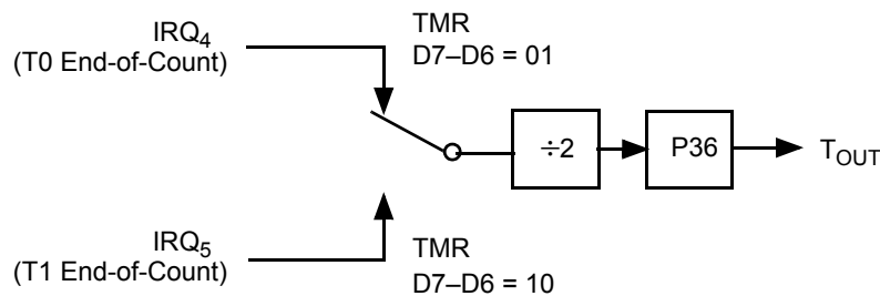
Figure 78. T0 and T1 Output Through T_{OUT}
