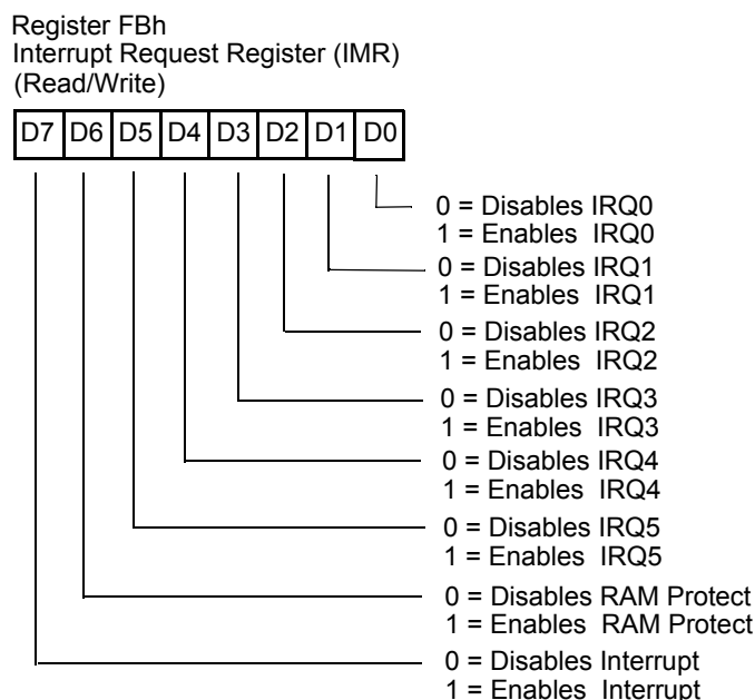
Figure 97. Interrupt Mask Register
