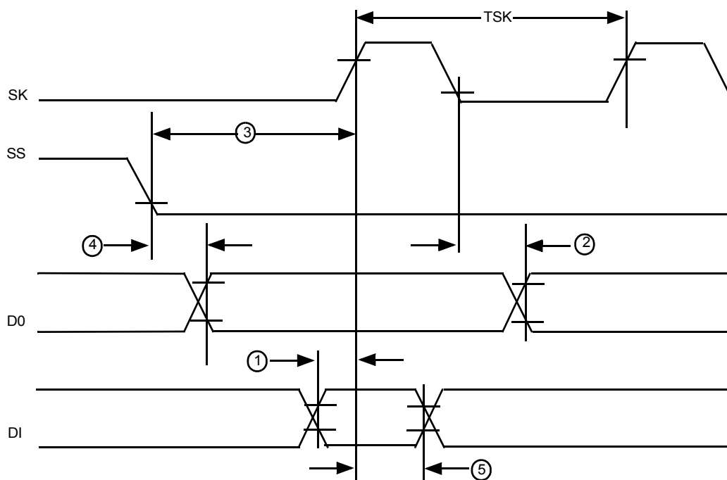
Figure 118. SPI Timing
