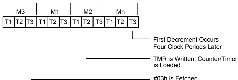
Figure 75. Counting Modes
