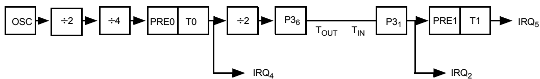
Figure 85. Cascaded Counter/Timers
