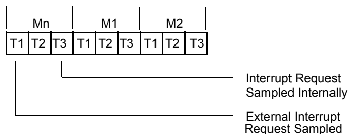
Figure 95. Interrupt Request Timing
