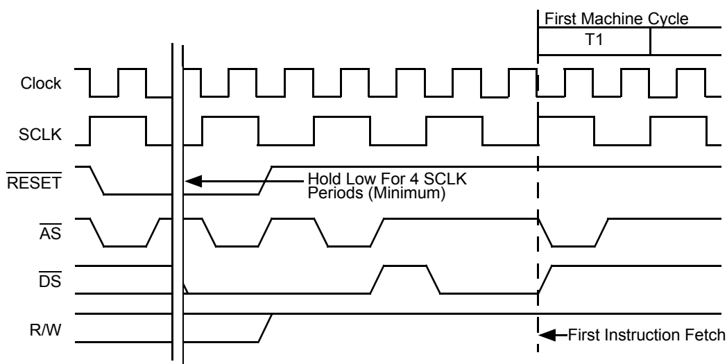
Figure 22. Reset Timing
