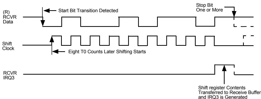
Figure 110. Receiver Timing
