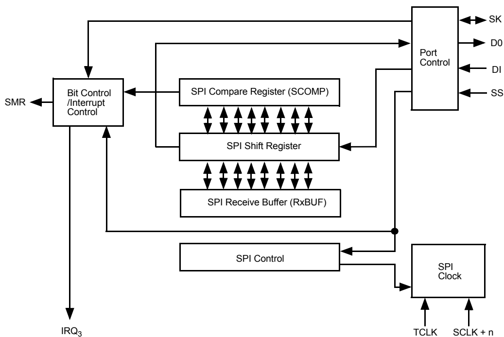
Figure 119. SPI Logic
