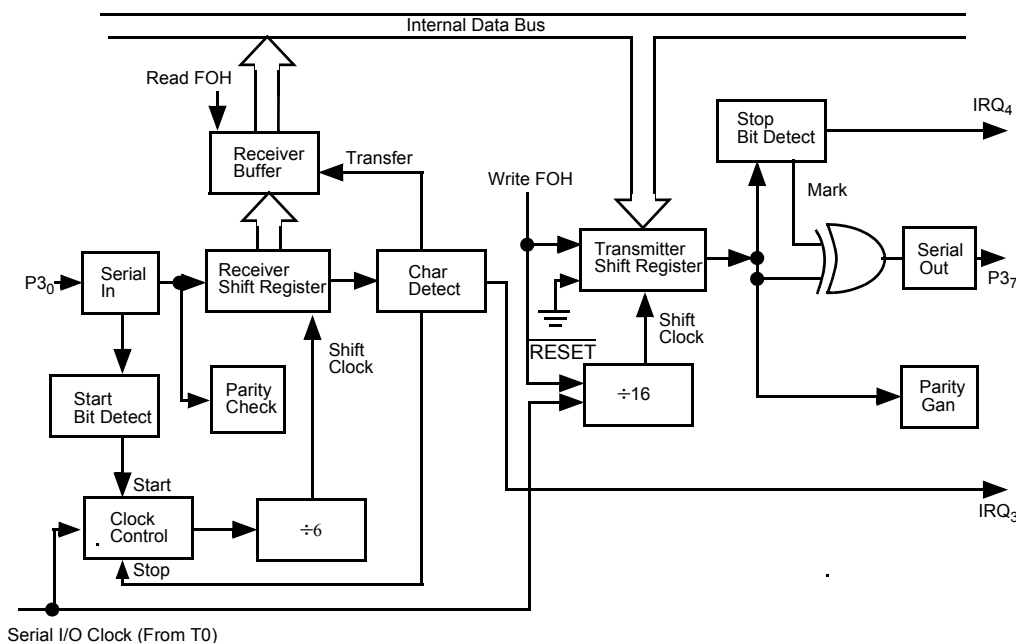
Figure 105. UART Block Diagram
