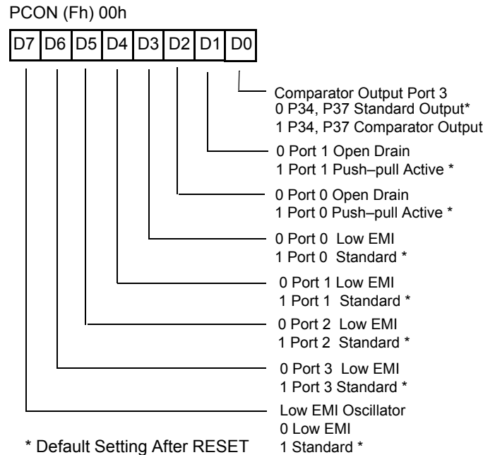
Figure 62. Port Configuration Register (Write-Only)
