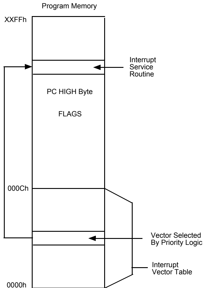
Figure 101. Interrupt Vectoring
