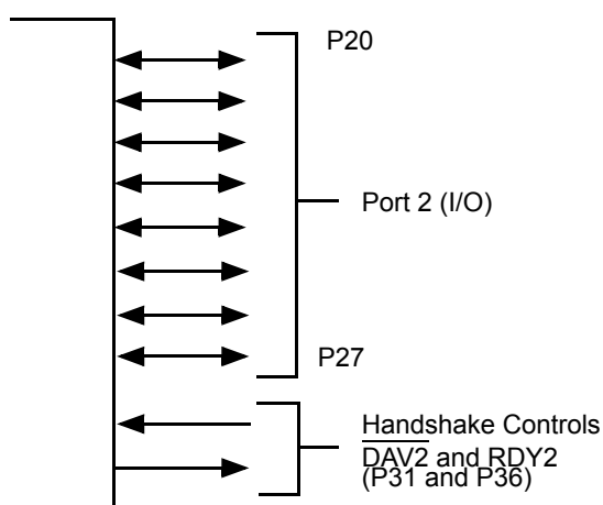
Figure 43. Port 2 Handshaking
