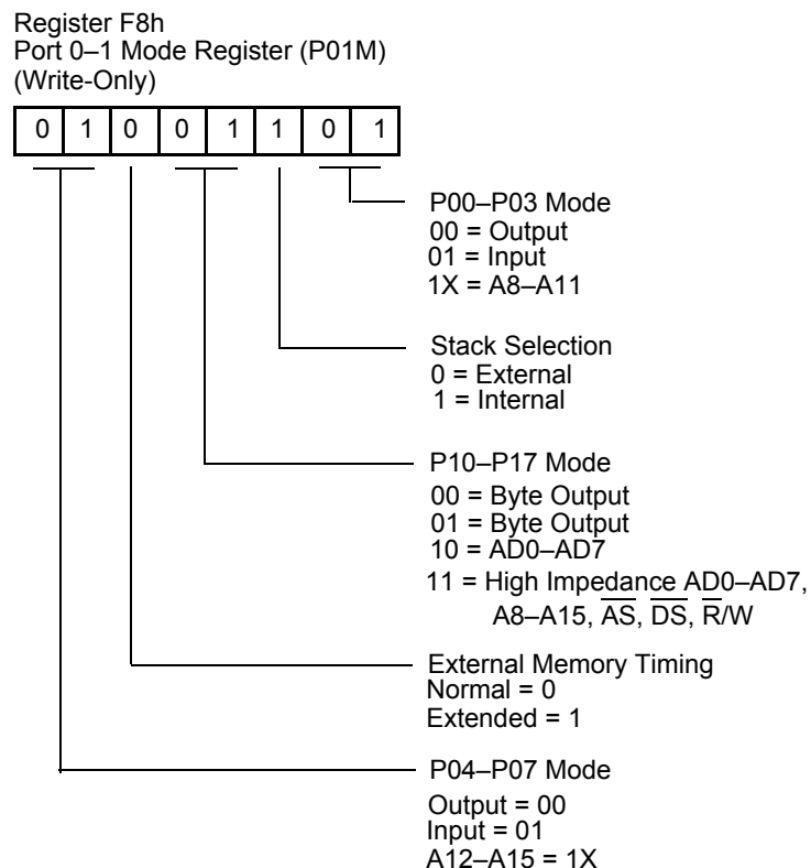
Figure 54. Port 0/1 Reset
