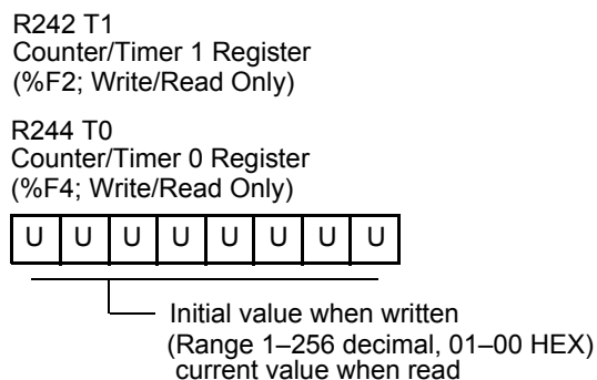
Figure 86. Counter/Timer Reset
