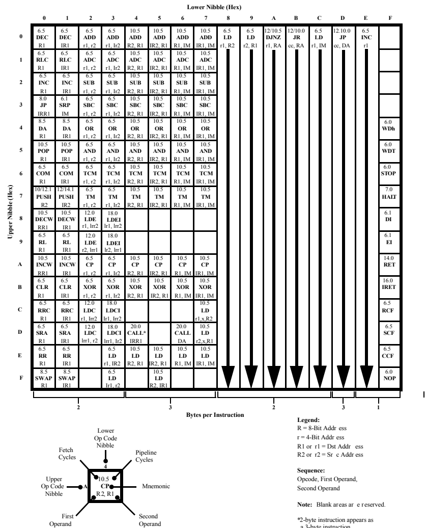
Figure 134. Op Code Map
