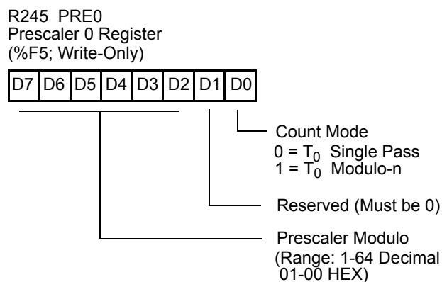
Figure 70. Prescaler 0 Register
