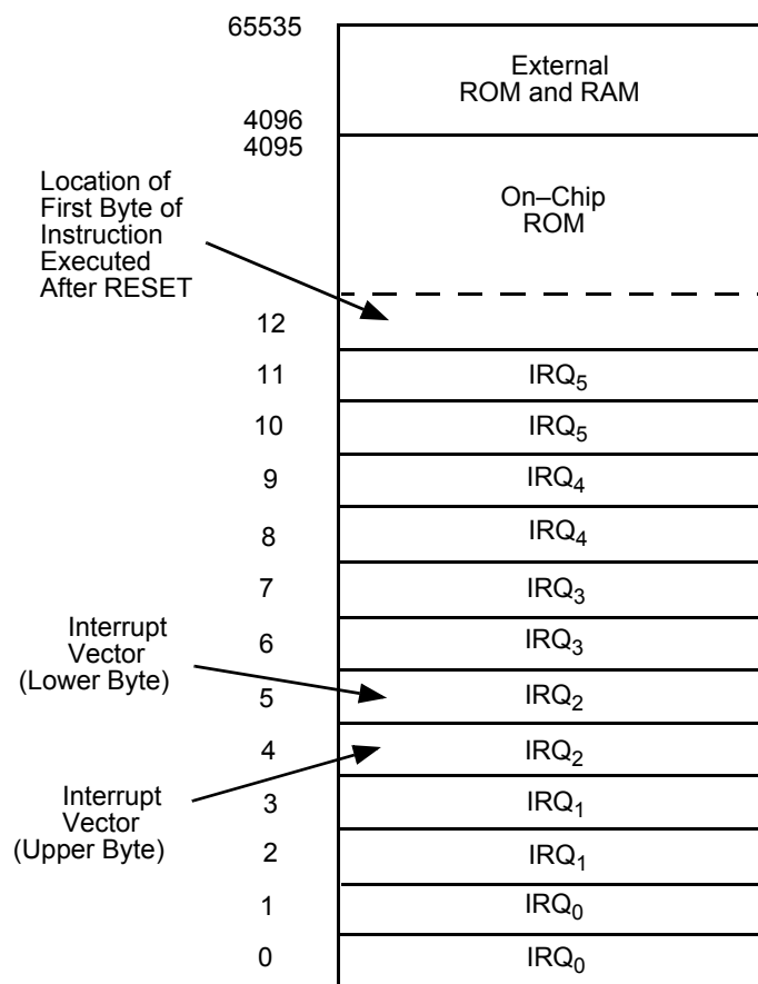
Figure 8. Z8 Program Memory Map
