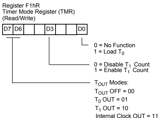
Figure 76. Timer Mode Register ( T_{OUT} Operation)
