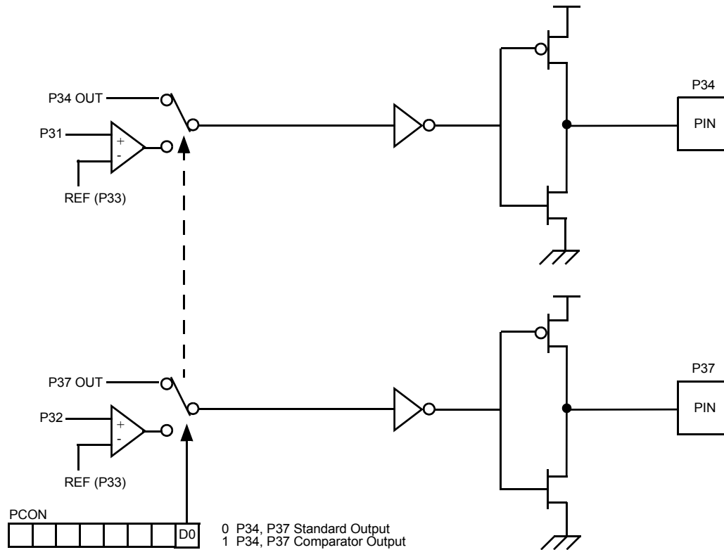
Figure 60. Port 3 Configuration
