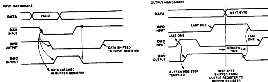
Figure 8. 3-Wire Handshake
