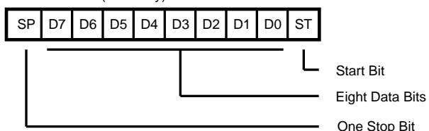
Received Data (No Parity)
