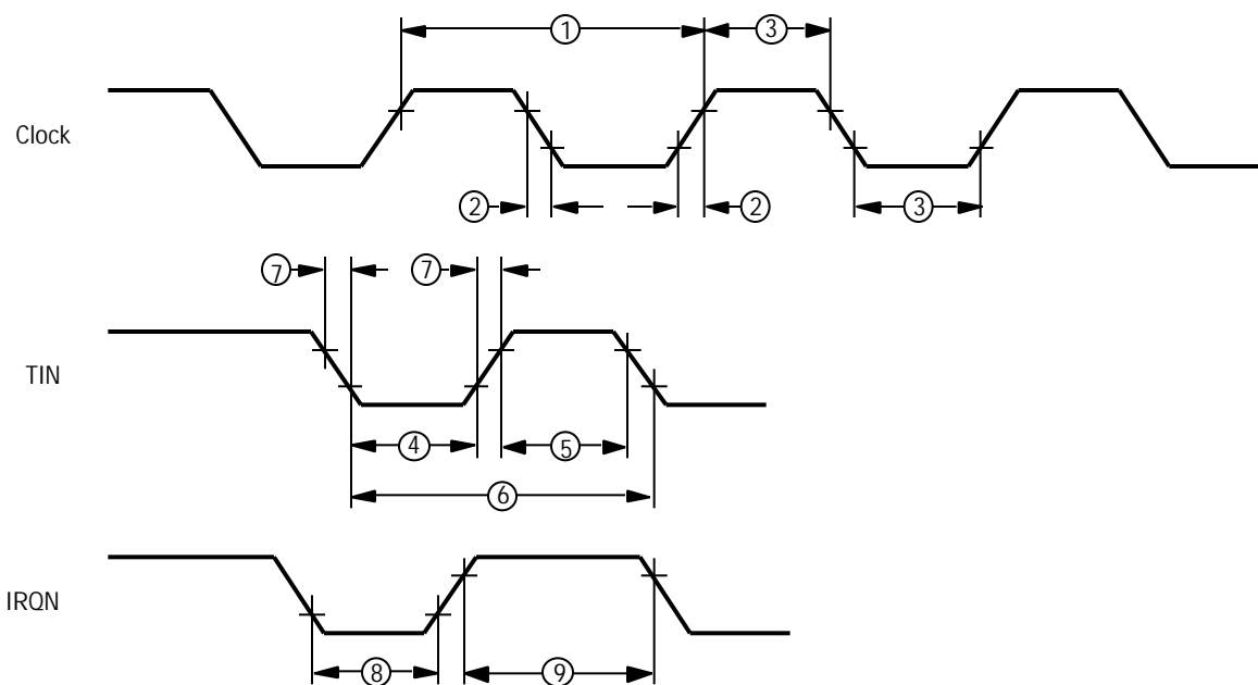
Figure 20. Additional Timing
