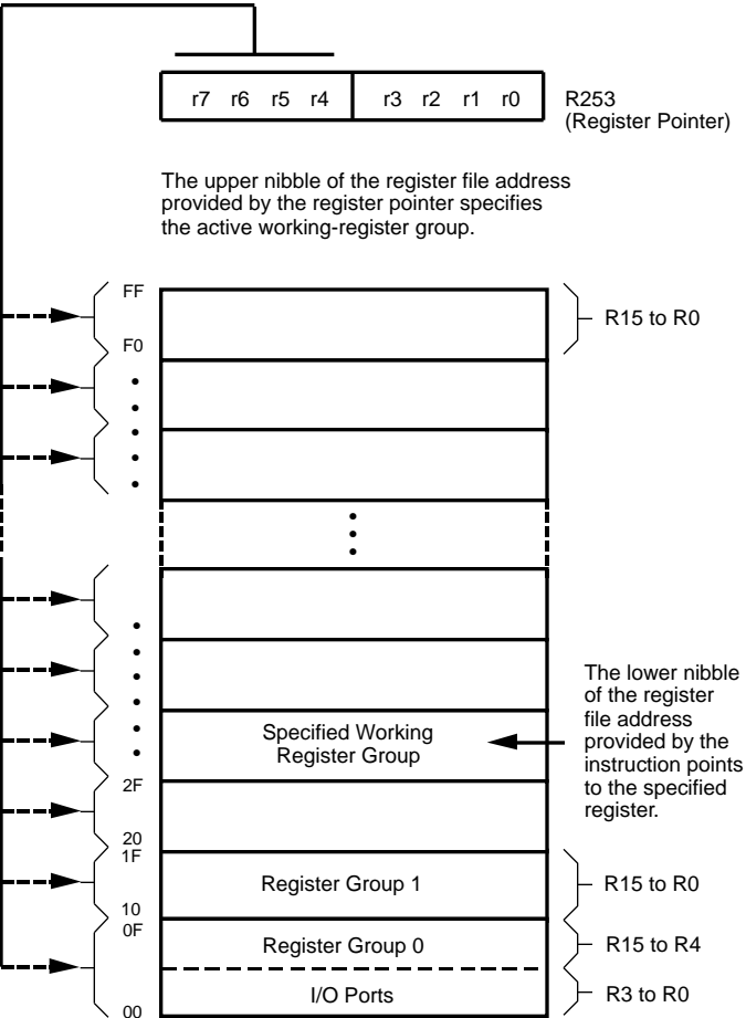
Figure 13. Register Pointer
