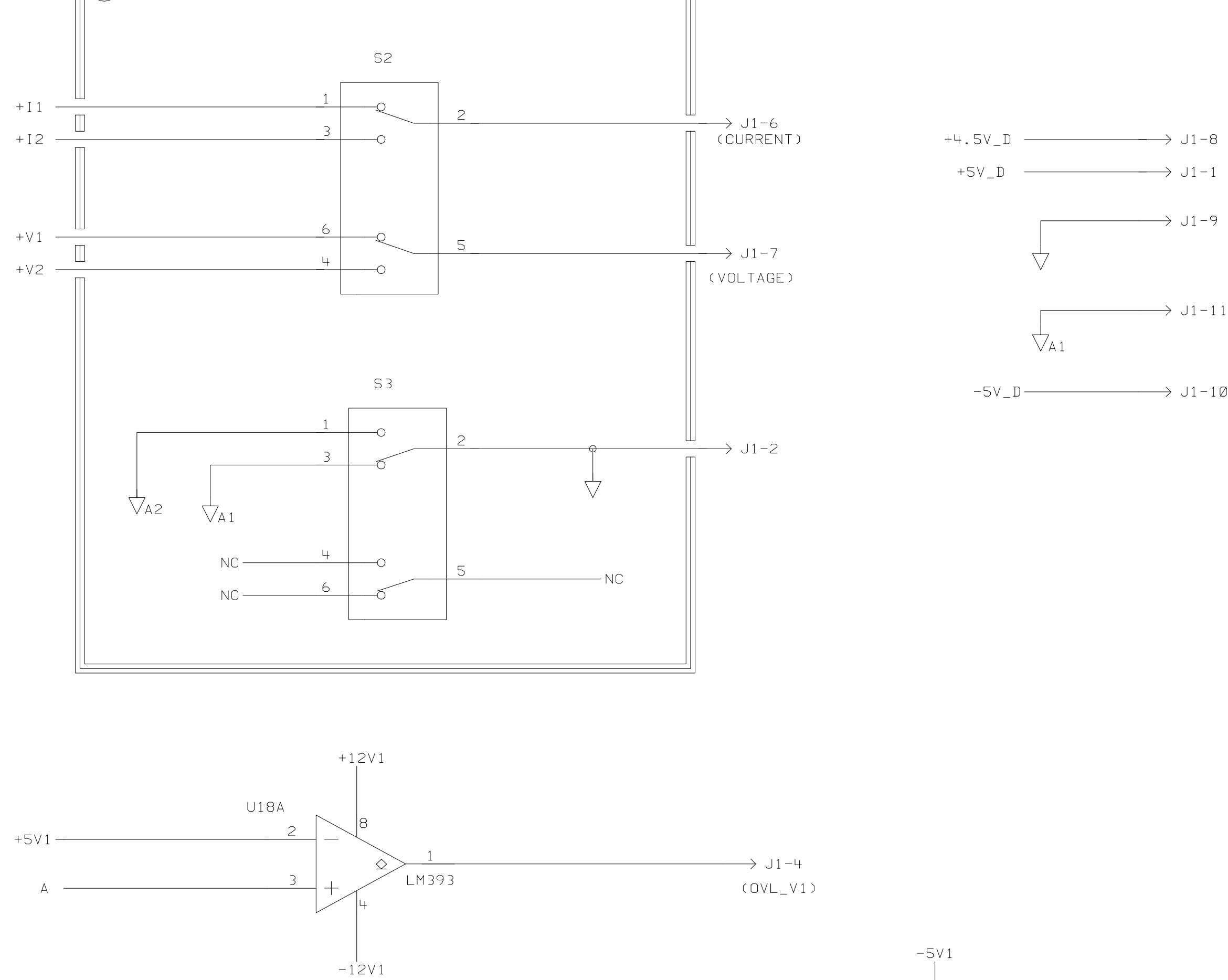
Ⓒ Meter Select Circuit
