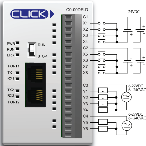
Wiring Diagram
