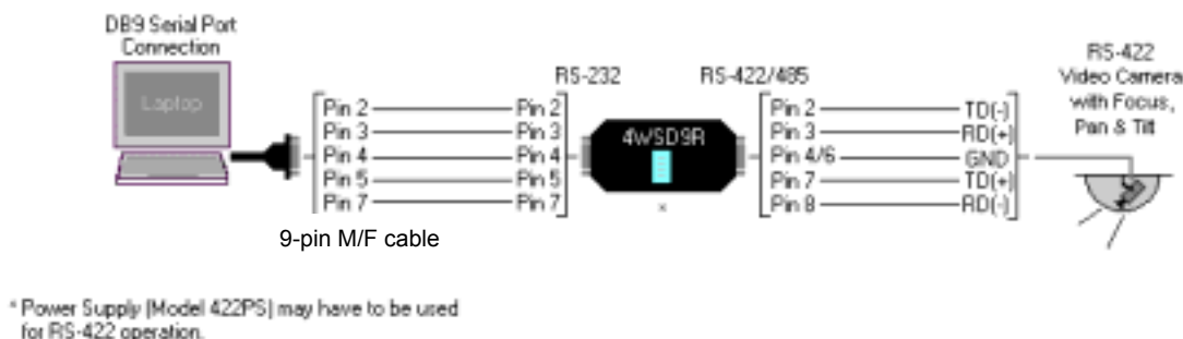
Figure 3: RS-422 4-wire full-duplex diagram
