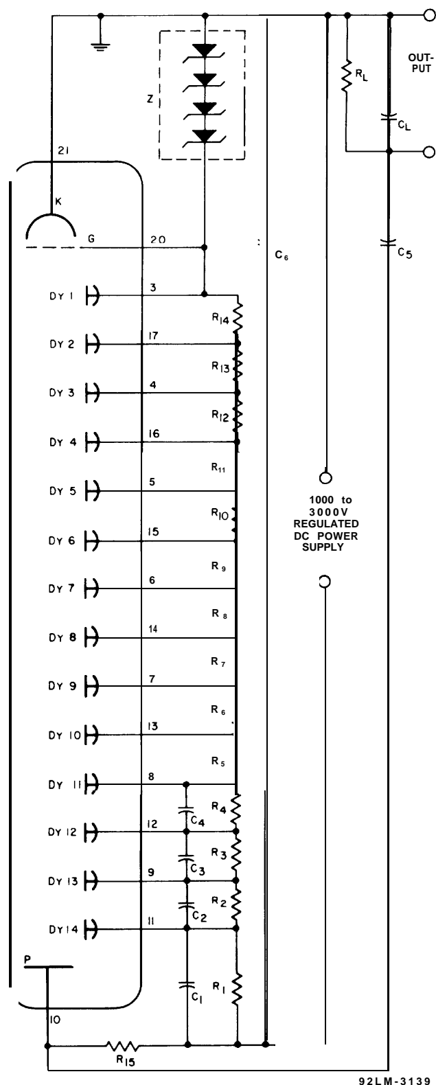
Figure 9 - Typical Circuit Arrangement for Scintillation-Counting Applications
