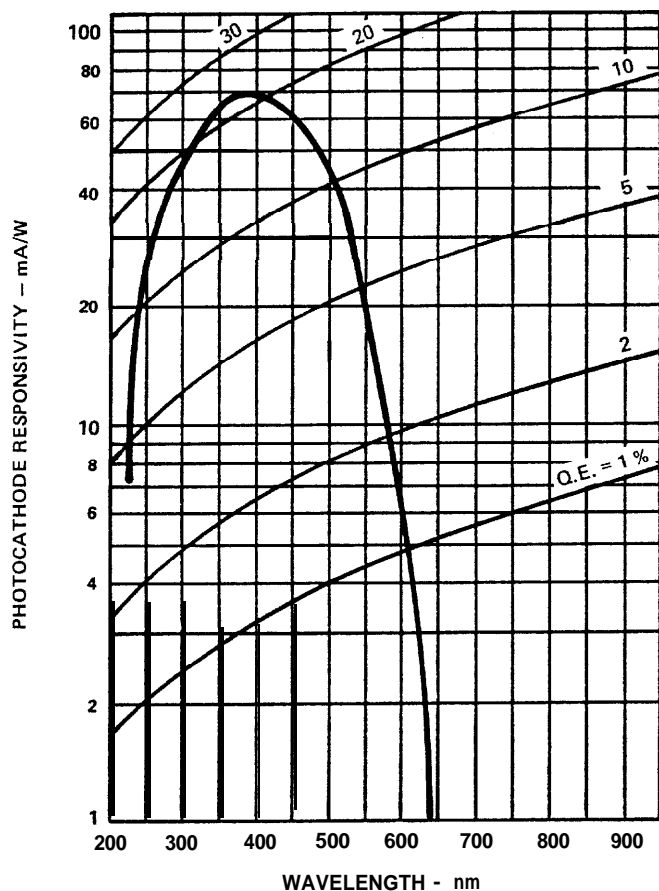
Figure 1 - Typical Spectral Response Characteristics
