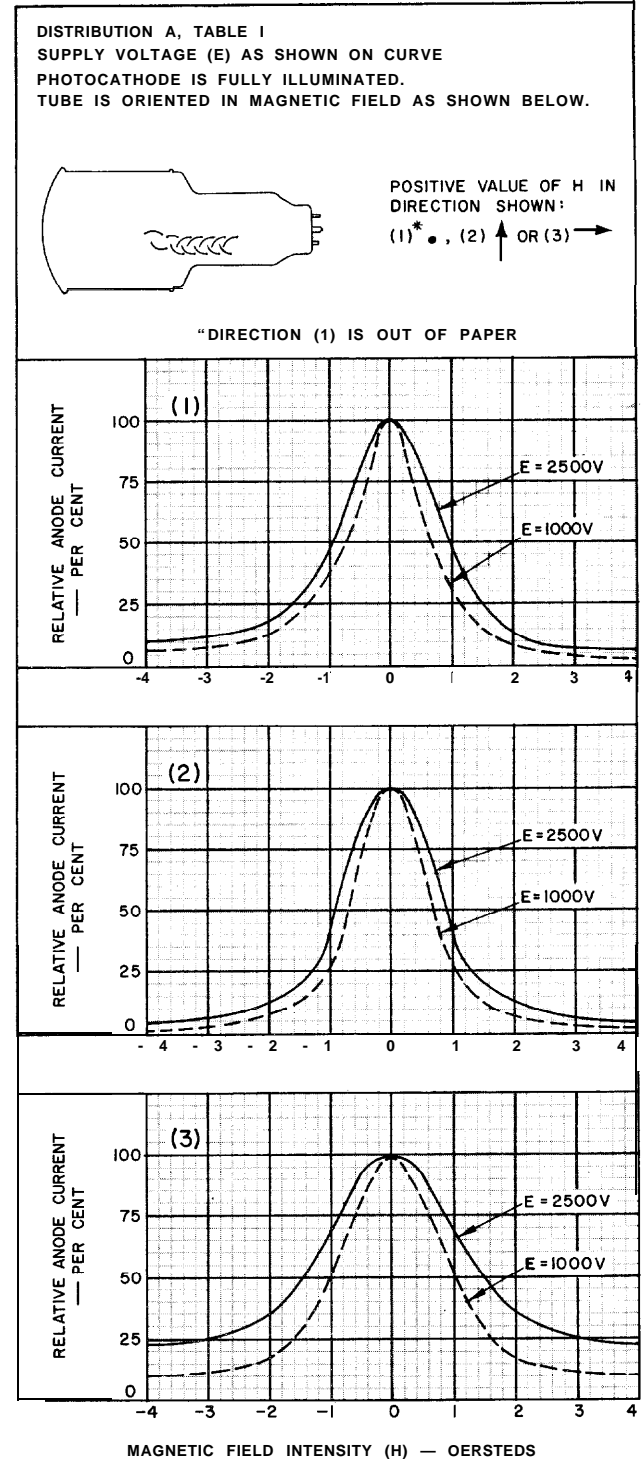
Figure 8 - Typical Effect of Indicated Magnetic Field on Anode Current
