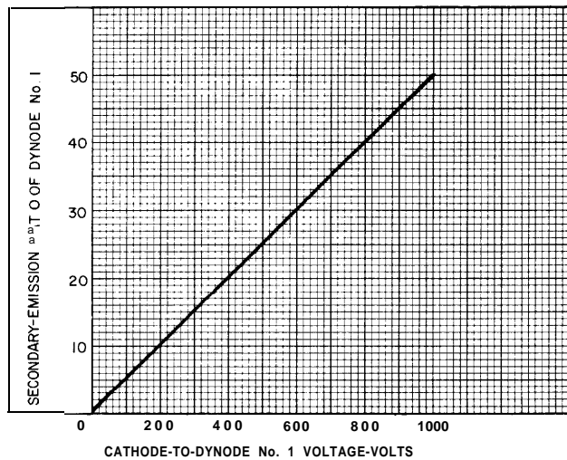
Figure 4 - Typical Secondary-Emission Ratio of First Dynode as a Function of Cathode-to-Dynode No.1 Voltage
