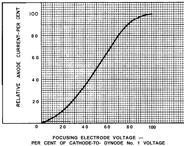
Figure 5 - Typical Focusing Electrode Characteristic
