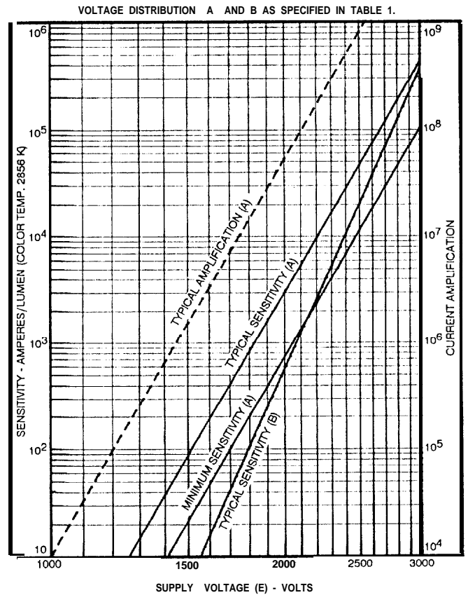
Figure 6 - Sensitivity and Current Amplification Characteristics
