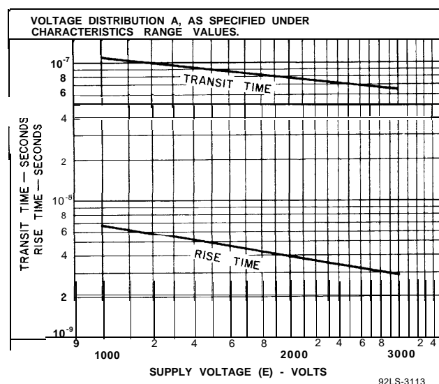
Figure 3 - Typical Time Resolution Characteristics
