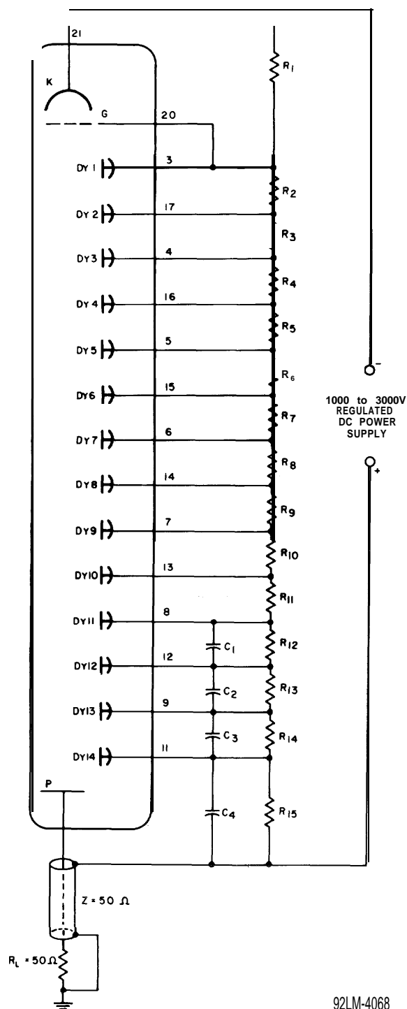
Figure 10 - Typical Circuit Arrangement for Fast Pulse Response and High Peak Current Application
