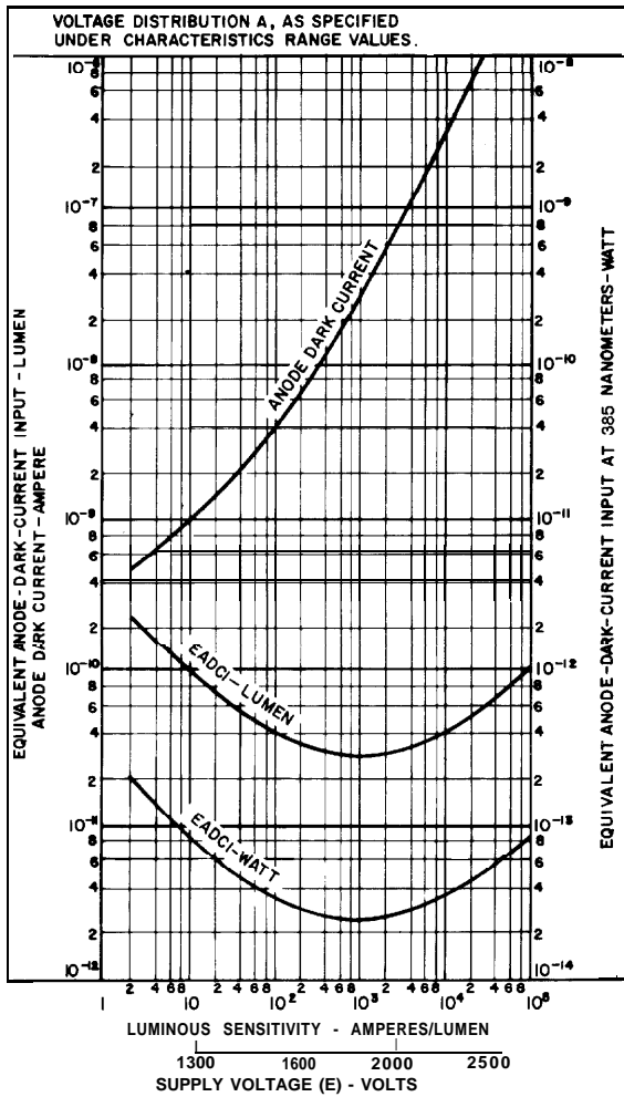
Figure 7 - Typical EADCI and Anode Dark Current Characteristics
