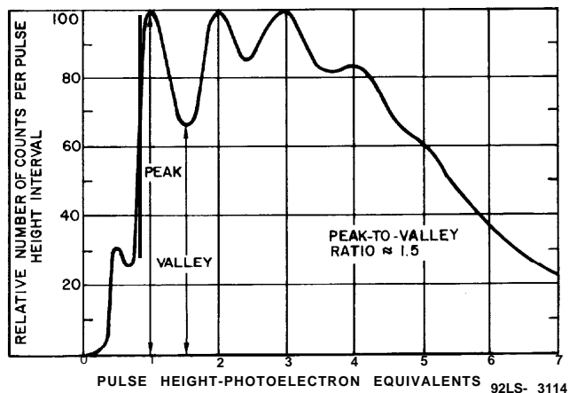
Figure 2 - Typical Photoelectron Pulse Height Spectrum
