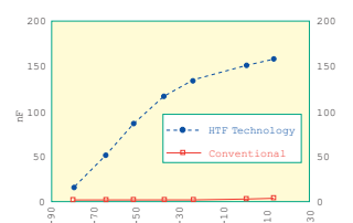
Hyper Thin Film vs. Conventional Sensor Change of Capacitance with Dewpoint
