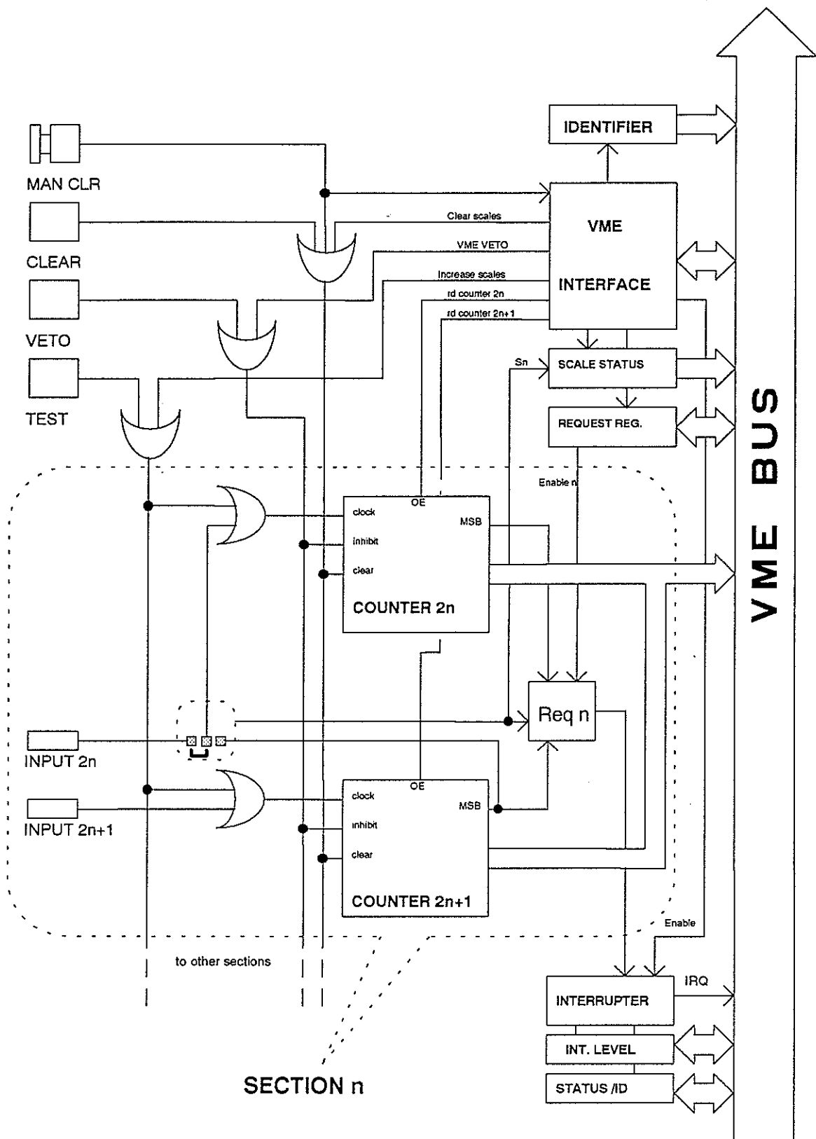
Fig. 1.1: Mod. V560 block diagram
