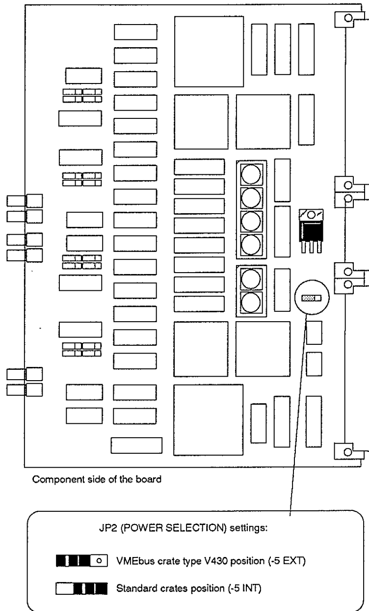
Fig. 3.1: Mod. V560 JP2 settings
