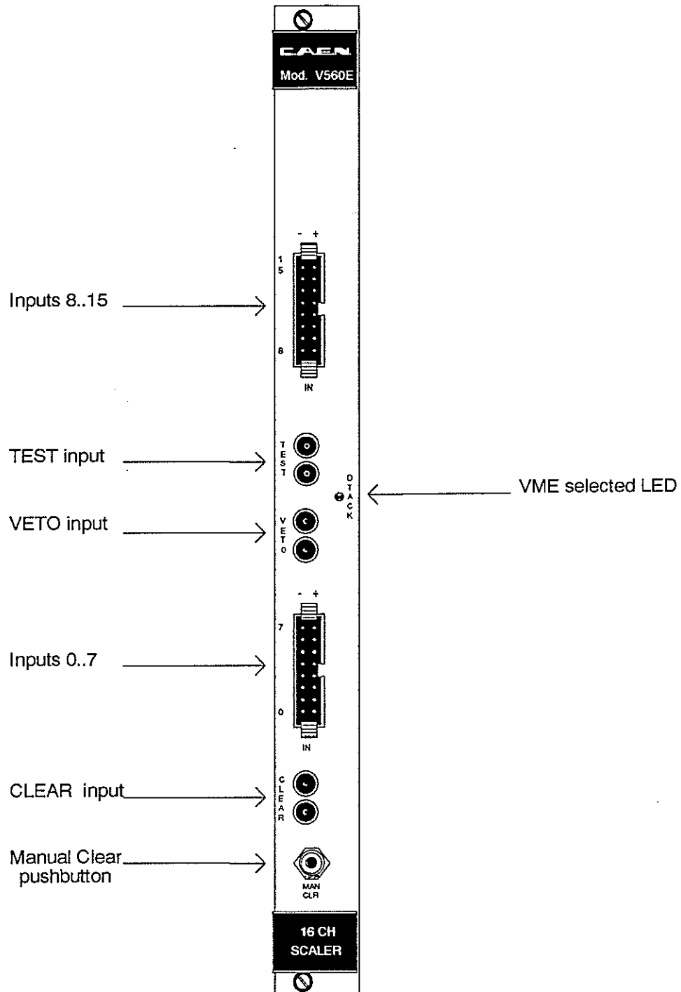
Fig. 2.1: Mod. V560 Front panel
