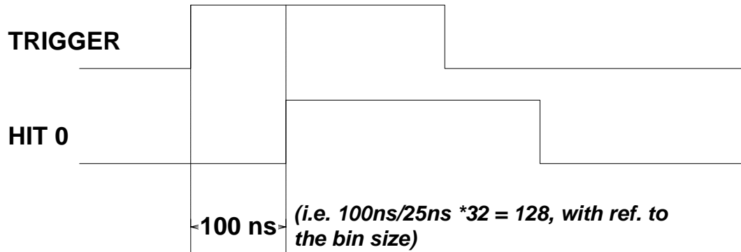
Fig. 5.3: TRIGGER and HIT 0 signals to test Stop Trigger Matching operation mode
