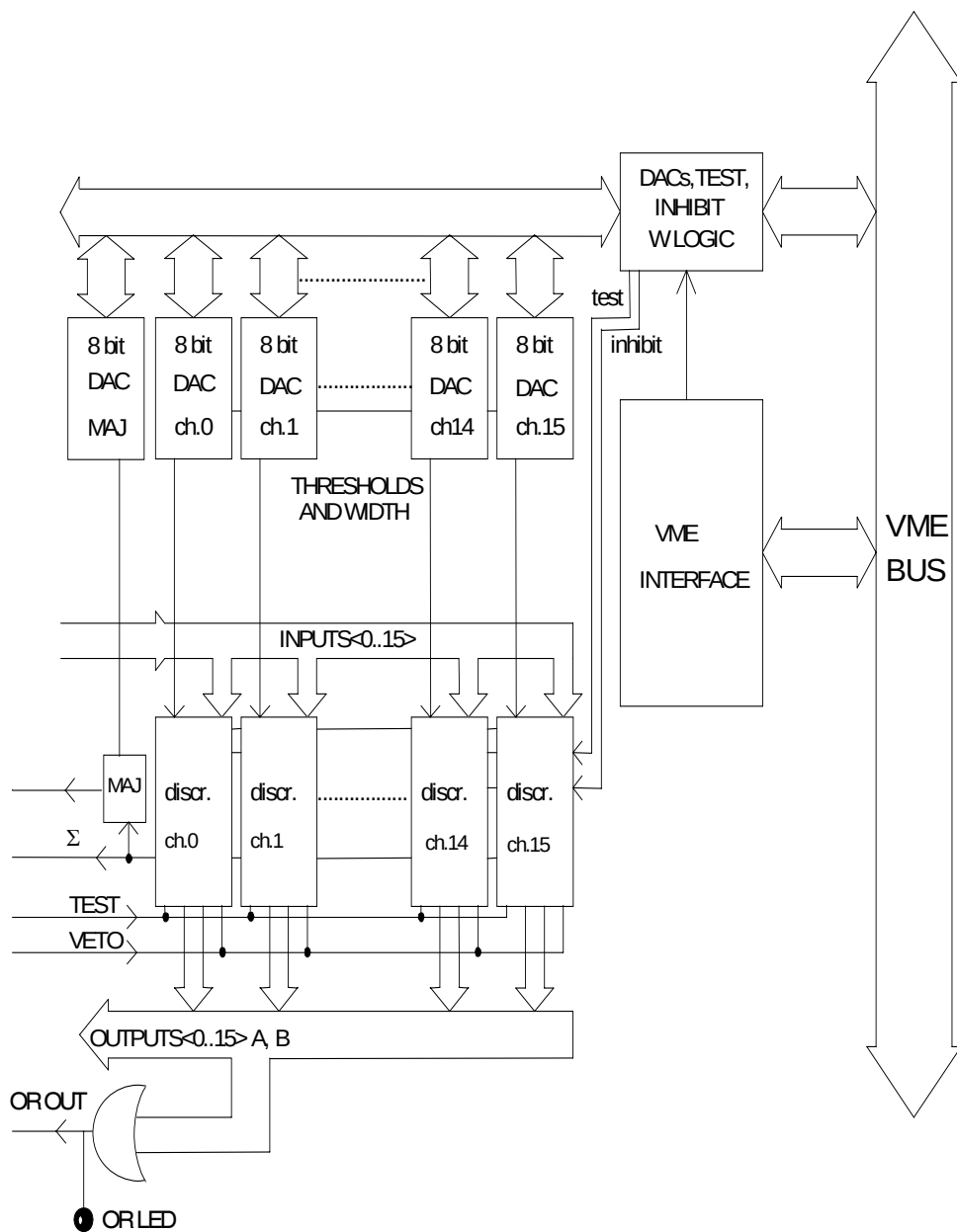
Fig. 1.2: Block Diagram
