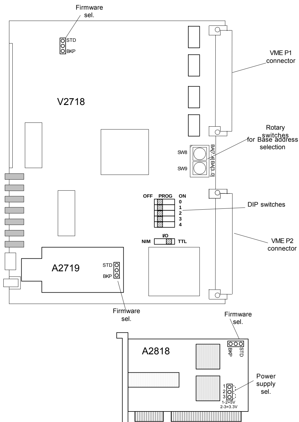
Fig. 3.3: Component Location
