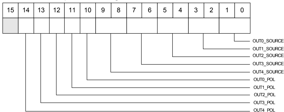
Fig. 2.14: Output Multiplexer Set register
