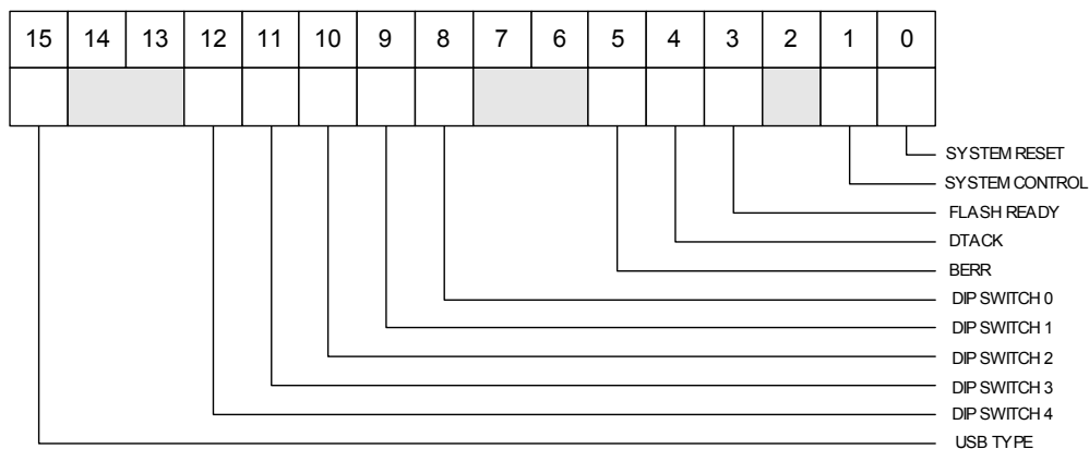
Fig. 2.4: Status Register
