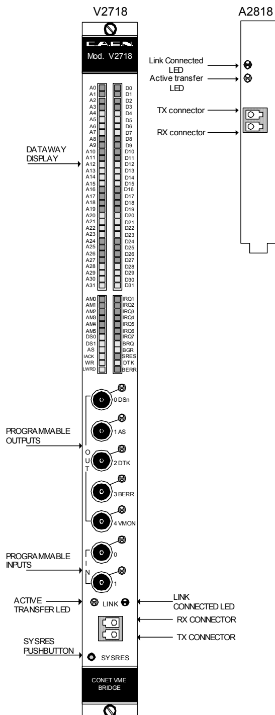
Fig. 3.1: Mod. V2718 and A2818 front panels
