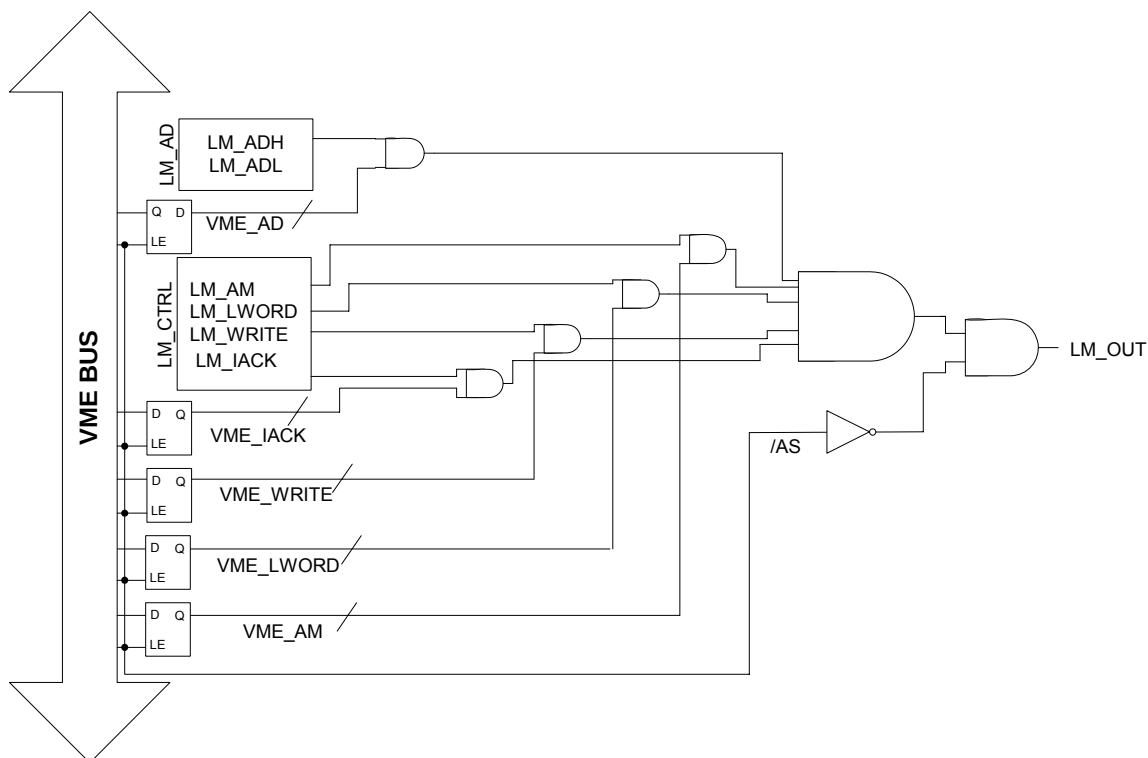
Fig. 2.3: The Location Monitor
