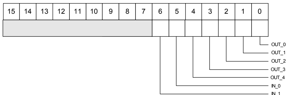
Fig. 2.17: LED polarity clear register
