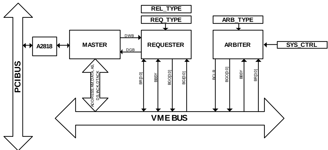
Fig. 2.1: Internal Arbitration for VME bus Requests
