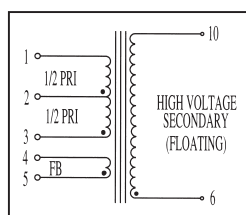
Schematic C
