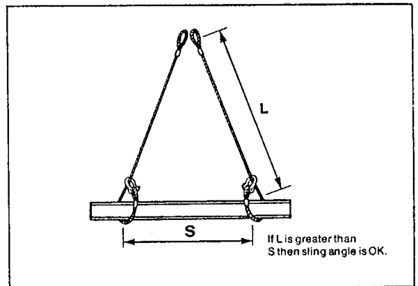
Check on Sling Angle
