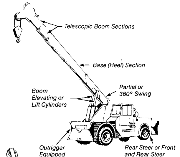
PICK AND CARRY
