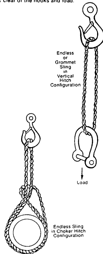
ENDLESS OR GROMMET SLINGS
