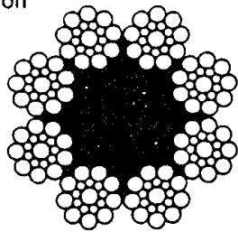
8x19 Seale, Fibre Core
