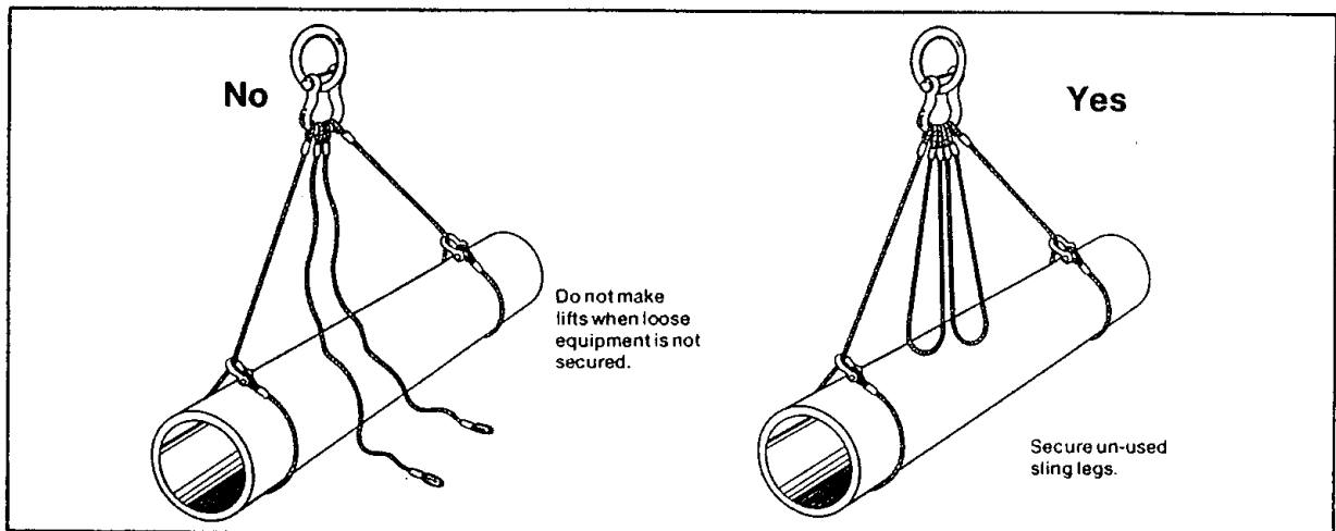
Secure All Unused Sling Legs
