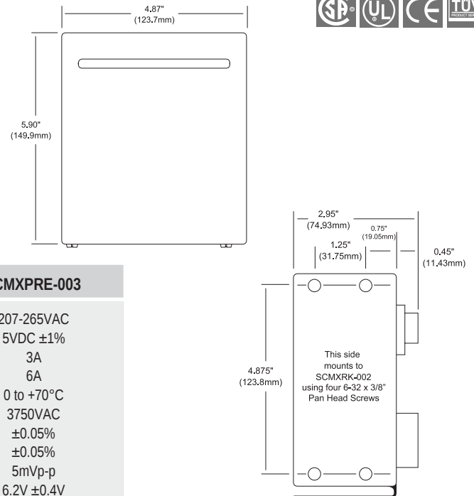
Figure 26: SCMXPRT-003/SCMXPRE-003 Physical Dimensions
