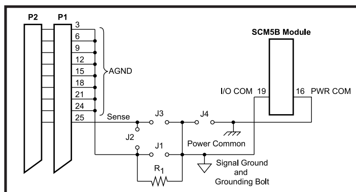
Figure 4: SCMPB01 Grounding Diagram
