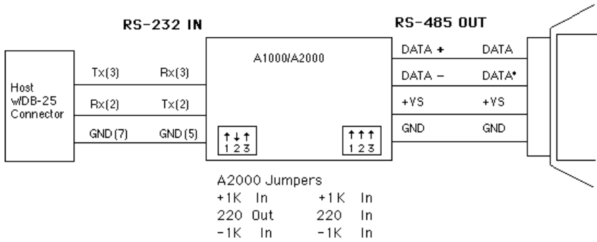
Figure 4a Wiring diagram for RS-232/RS-485 converter with host DB-9 connector.
