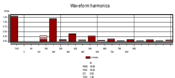
Figure 10 Harmonics Spectrum
