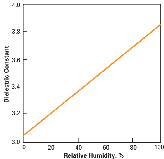
Figure 13. Dielectric Constant vs. Relative Humidity, Type HN Film, 25 µm (1 mil)
