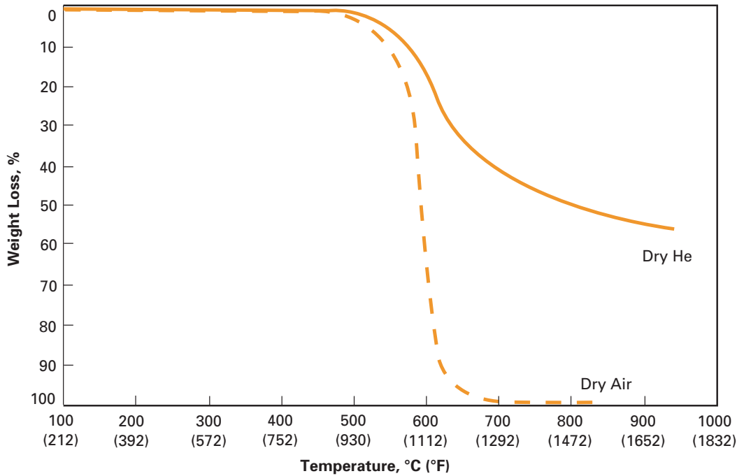
Figure 9. Weight Loss, Type HN Film, 25 µm (1 mil)*
