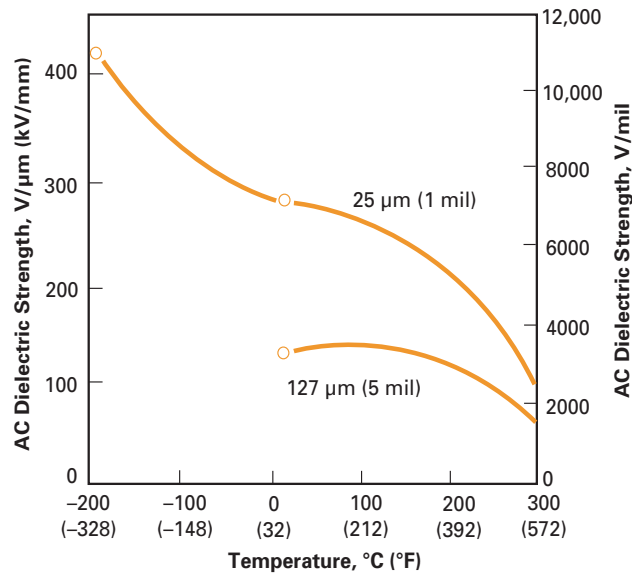
Figure 14. AC Dielectric Strength vs. Temperature, Type HN Film, 25 µm (1 mil)
