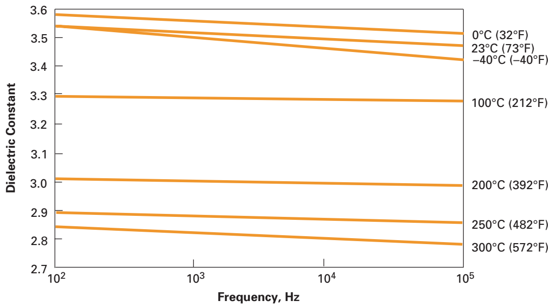
Figure 18. Dielectric Constant vs. Frequency, Type HN Film, 25 µm (1 mil)
