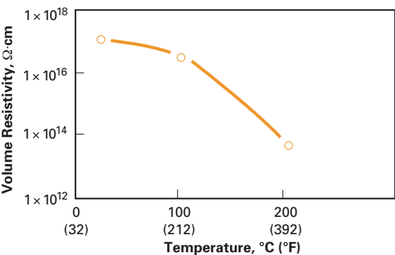
Figure 17. Volume Resistivity vs. Temperature, Type HN Film, 25 µm (1 mil)
