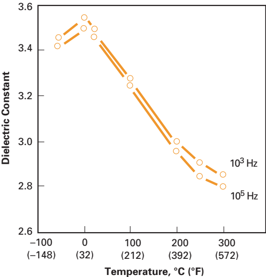
Figure 15. Dielectric Constant vs. Temperature, Type HN Film, 25 µm (1 mil)
