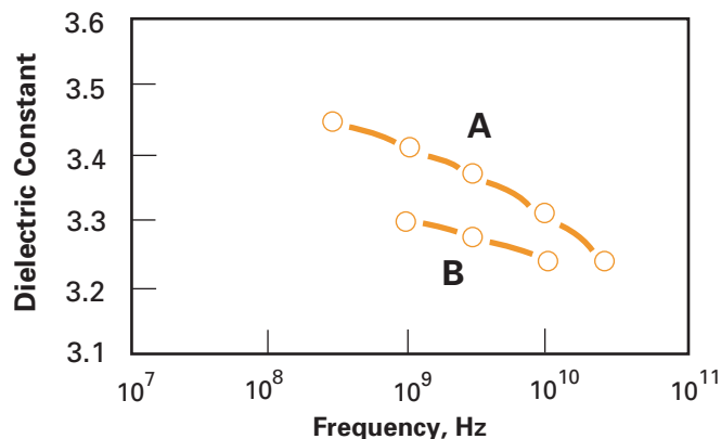
Figure 20. Dielectric Constant vs. Frequency, Type HN Film, 125 \mu m (5 mil)*
