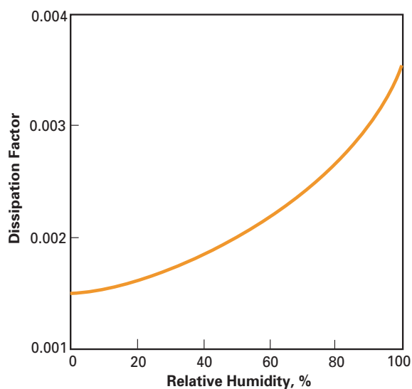
Figure 12. Dissipation Factor vs. Relative Humidity, Type HN Film, 25 µm (1 mil)
