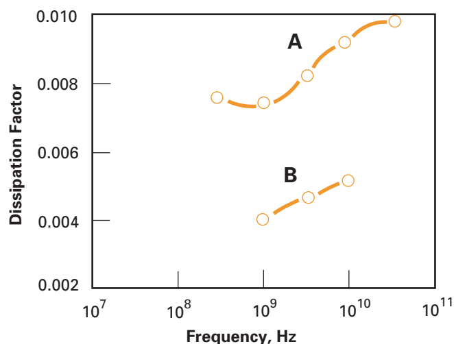
Figure 21. Dissipation Factor vs. Frequency, Type HN Film, 125 \mu m (5 mil)*
