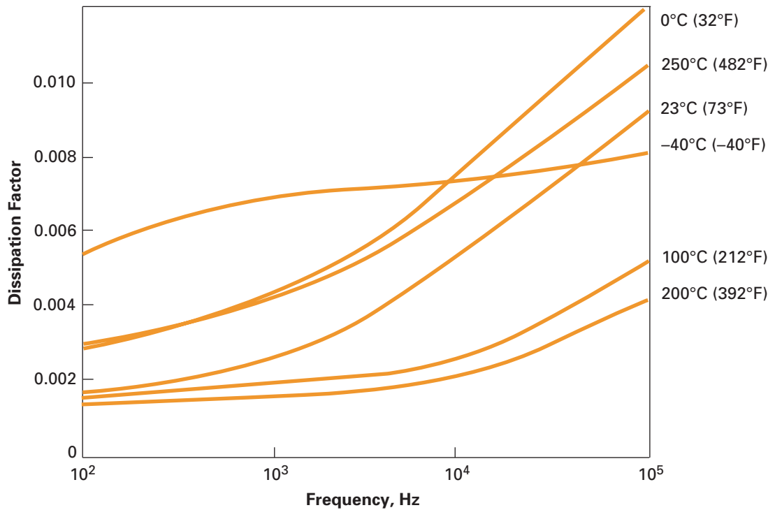
Figure 19. Dissipation Factor vs. Frequency, Type HN Film, 25 µm (1 mil)
