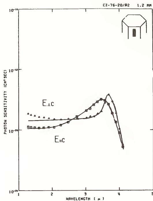
Fig.4 Photoconductive photon sensitivity, \Delta\sigma/(\sigma J_{ph}) , for two samples from photoconductive data of same thickness 1.2 mm, with the orientations E//c and E\perp c .
