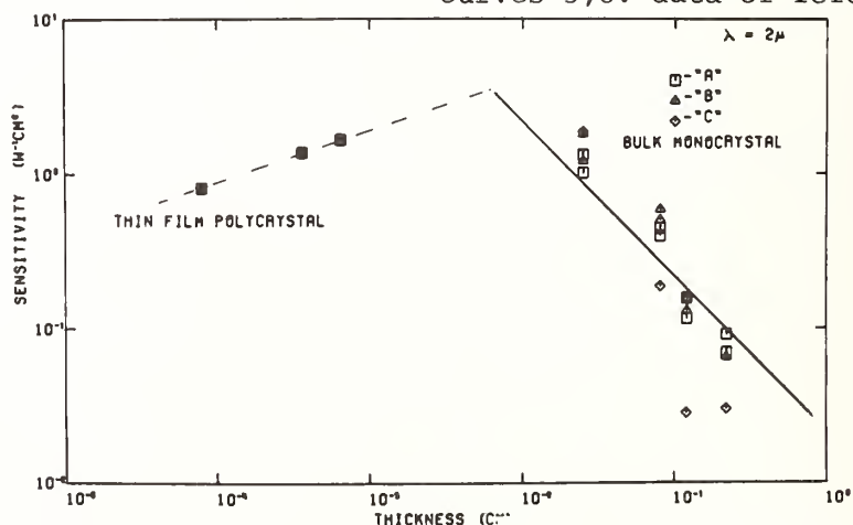
Fig.5 Photoconductive sensitivity, \Delta\sigma/(\sigma J) at \lambda=2\mu m plotted against sample thickness, d . The solid line for the bulk samples ( E\perp c ) corresponds to a 1/d variation.
