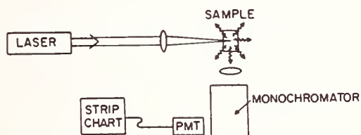
Fig. 2. Experimental setup.
