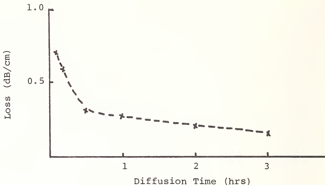
Fig. 1. Measured losses in waveguides fabricated by diffusion of evaporated silver at 500°C as a function of diffusion time.
