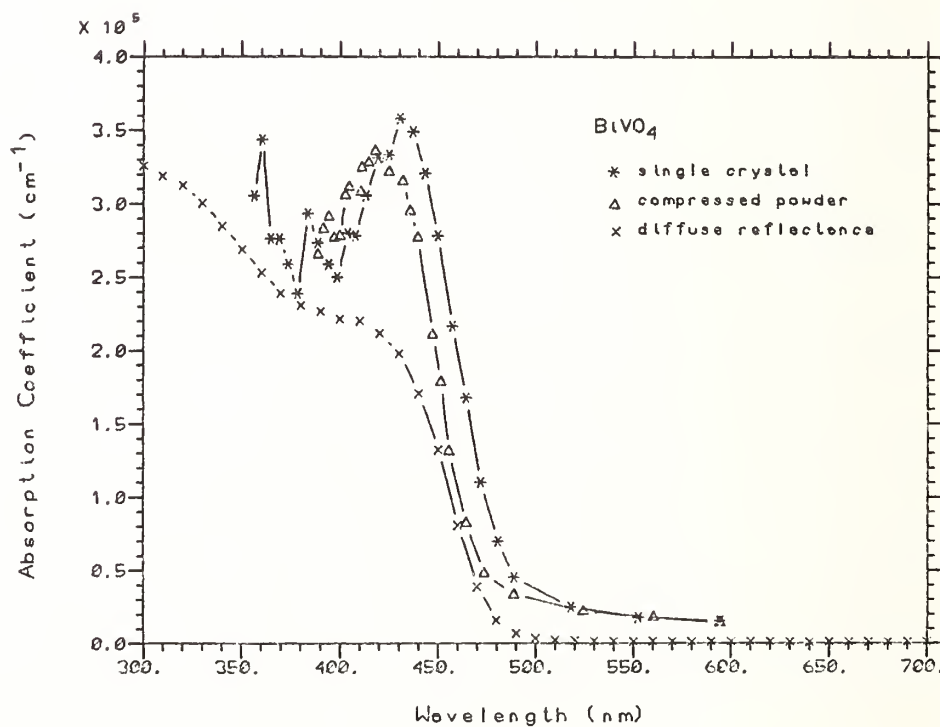
Fig. 1. Absorption coefficient vs. wavelength of \text{BiVO}_4 .
