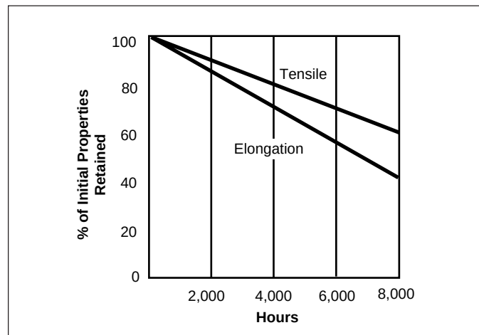
Figure 3. Accelerated Exposure (Atlas Sunshine Arc Weather-Ometer)
