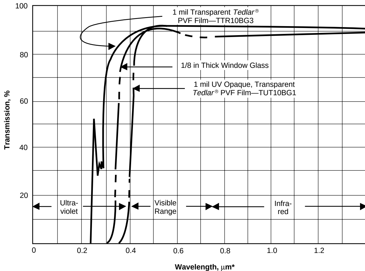
Figure 1. Spectral Transmission
