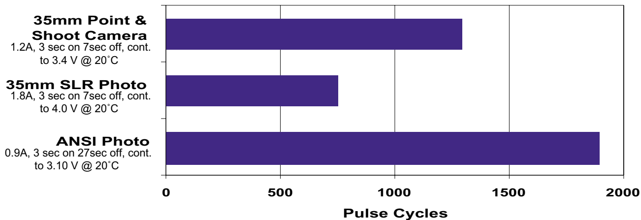
Duracell Ultra 223 Typical Performance
