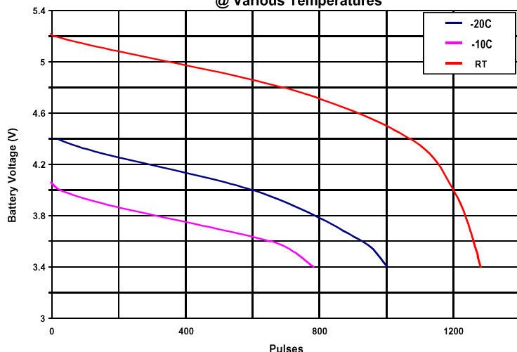
1.2 Amp, 3 sec on/ 7 sec off @ Various Temperatures
