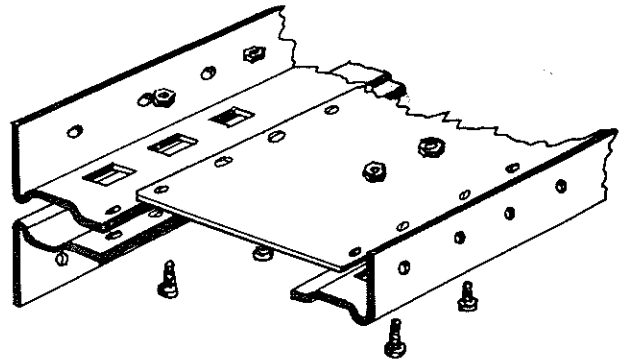
INTERMEDIATE ASSEMBLY
