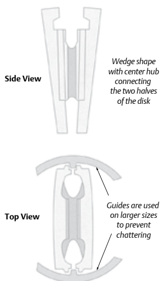
Figure 10.3 Flexible-Wedge Disk
