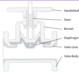
Figure 10.21 Straightway-Type Diaphragm Valve
