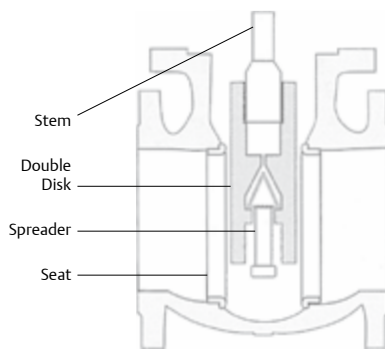
Figure 10.5 Double-Disk Gate Valve
