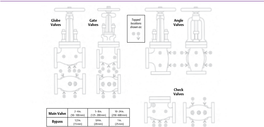
Figure 10.19 Bypass and Auxiliary Connections
