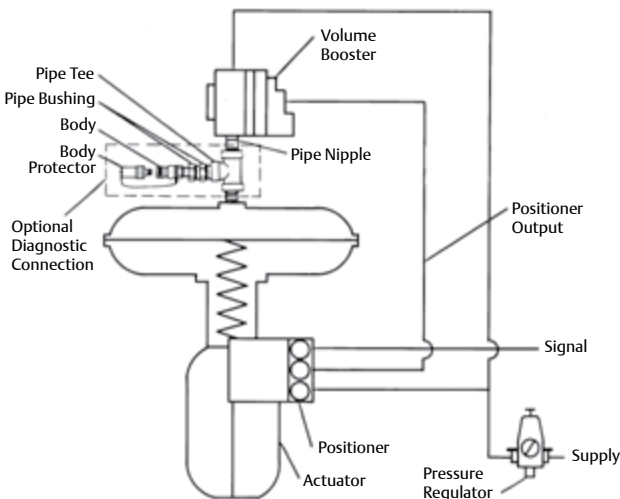
Figure 4.6 Typical Booster Installation with a Single-Acting Actuator
