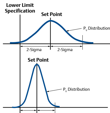
Figure 2.1 Process Variability
