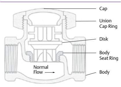
Figure 10.16 Horizontal-Lift Check Valve
