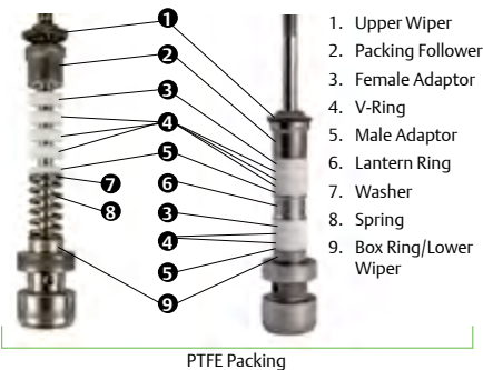
Figure 1.11 Packing
