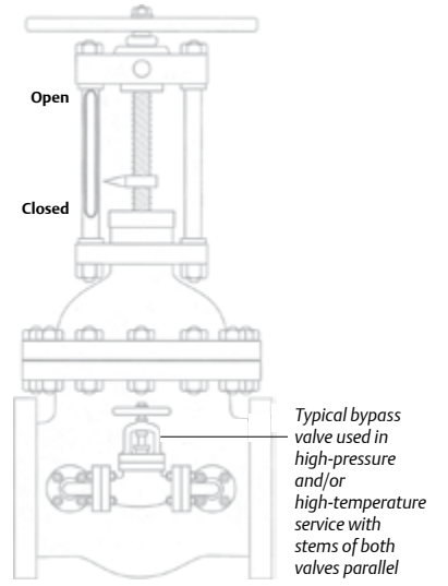
Figure 10.18 Bypass Valve
