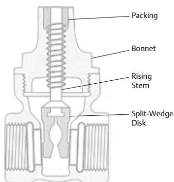
Figure 10.4 Split-Wedge Gate Valve
