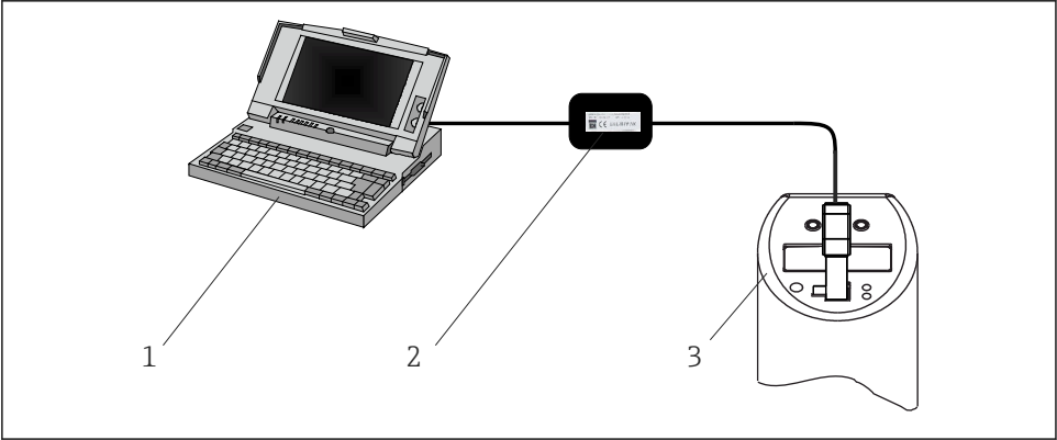
16 Operation, visualization and maintenance with PC and configuration software
