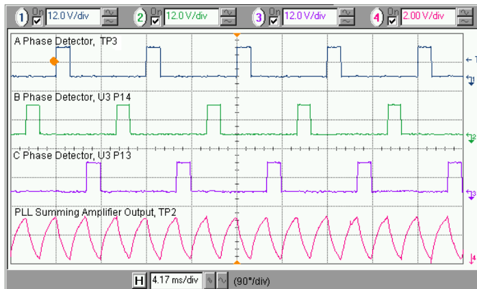
Figure 11. PLL Summing Amplifier Signals: \alpha=150^\circ
