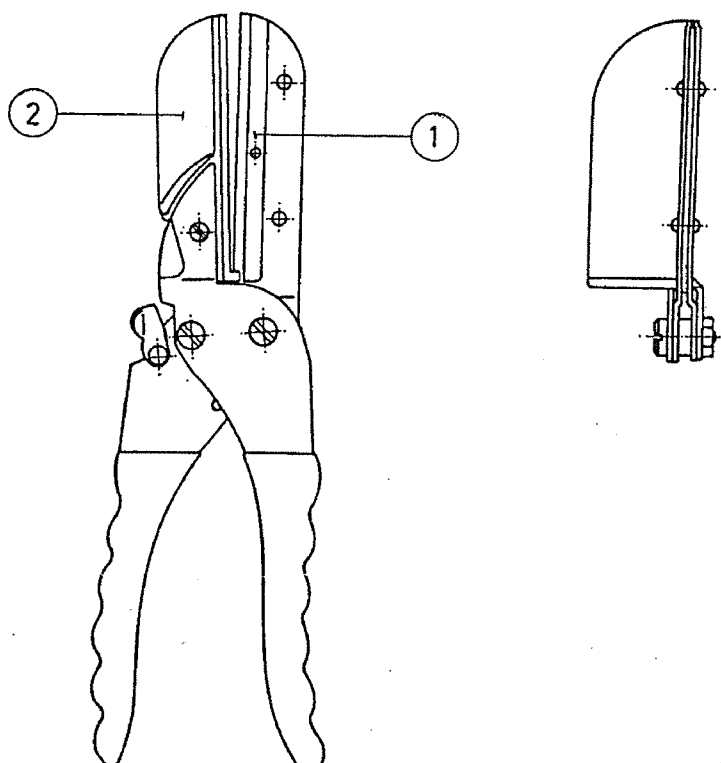
Figure 1: HT 209 Cable Shear Handtool
